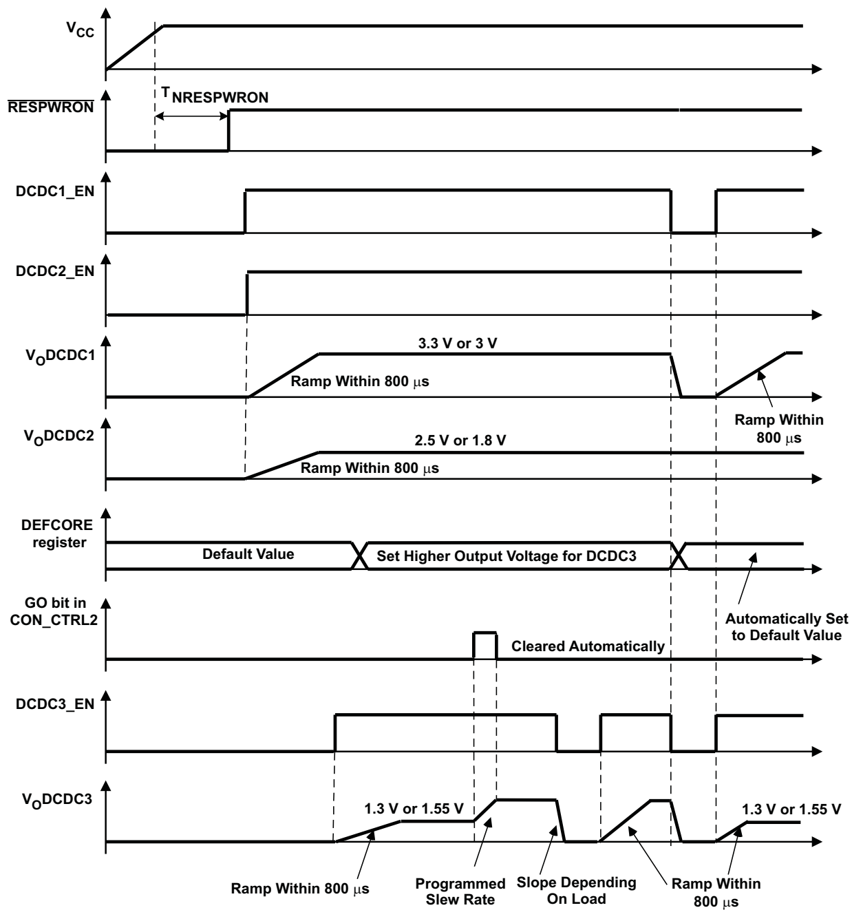
Figure 28. DVS Timing
