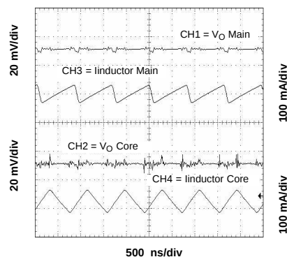
OUTPUT RIPPLE (PWM)
