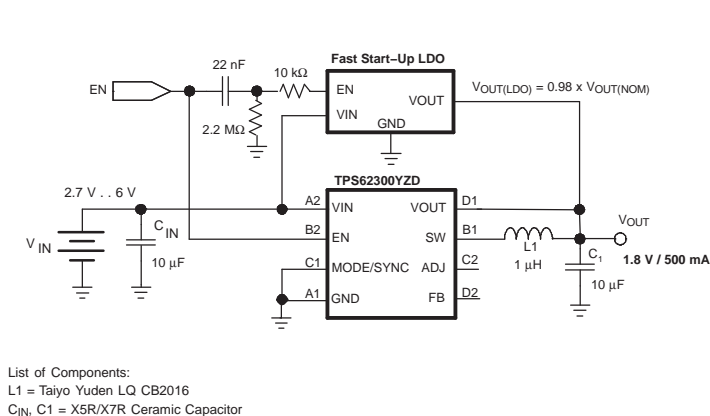
Figure 38. Speed-Up Circuitry for Fast Turnon Time
