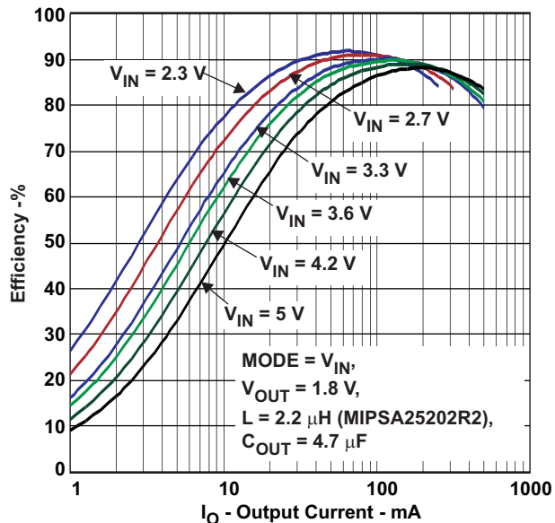
Figure 4. Efficiency Forced PWM Mode 1.8V Output voltage
