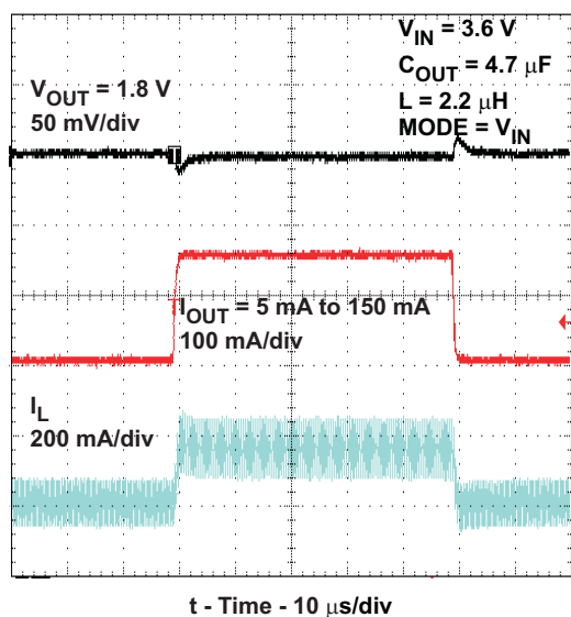
Figure 47. Load Transient Response 5mA to 150mA, Forced PWM Mode, V_{OUT} 1.8V
