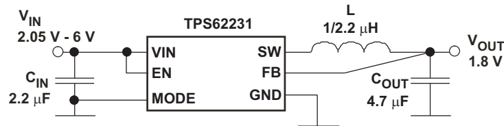
Figure 52. TPS62231 1.8V Output
