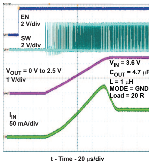
Figure 48. Start Up into 20Ω Load, V_{OUT} 2.5V
