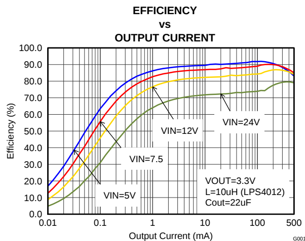
Figure 9. Vout=3.3V
