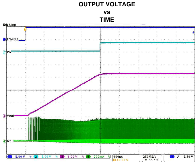
Figure 33. Startup into 100mA (VIN=12V, VOUT=3.3V)
