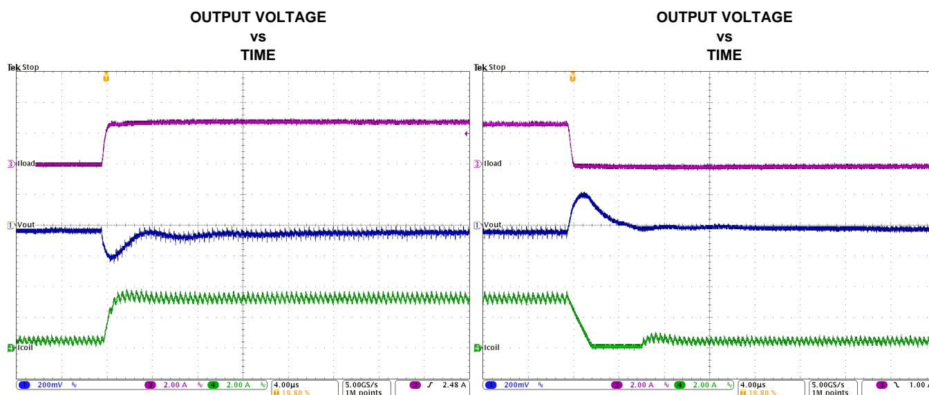
Figure 31. Load Transient Response of Figure 30, rising edge
