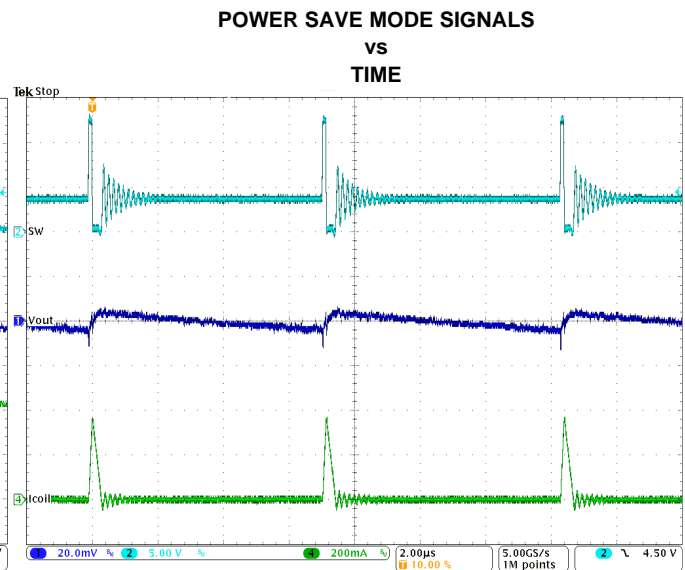
Figure 36. Typical Operation in Power Save Mode ( I_{OUT}=10mA )
