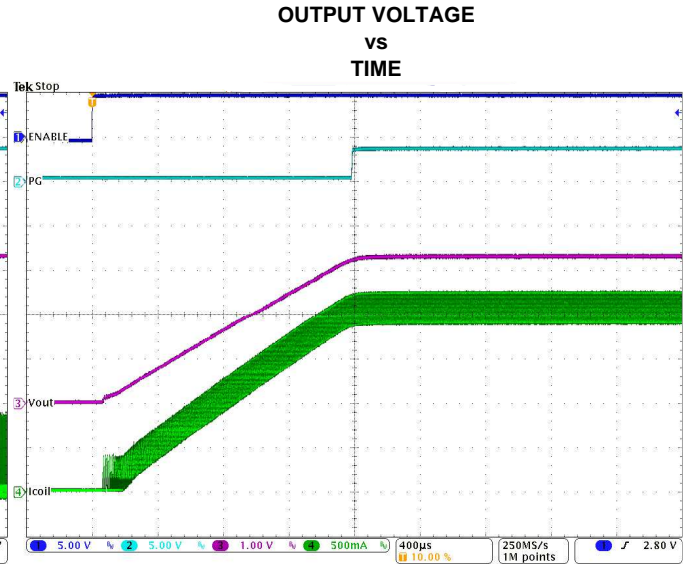
Figure 34. Startup into 3A (VIN=12V, VOUT=3.3V)
