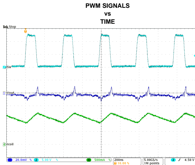
Figure 35. Typical Operation in PWM Mode ( I_{OUT}=1A )
