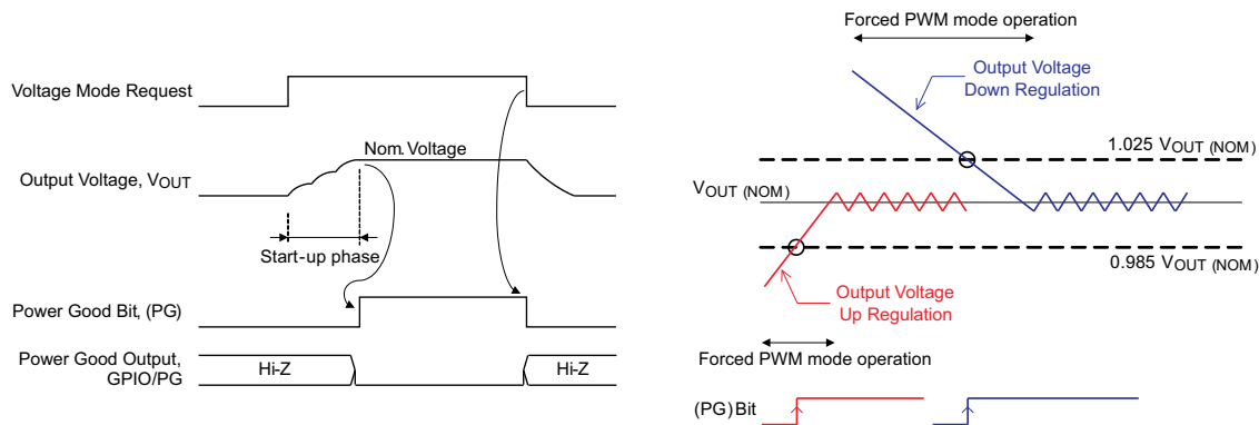
Figure 41. Power Good Operation ( \text{DIR} = 1 , \text{GPIOTYPE} = 1 )
