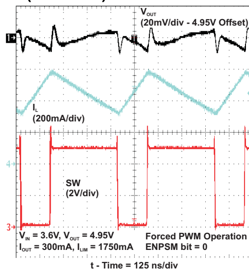
Figure 31. PWM OPERATION
