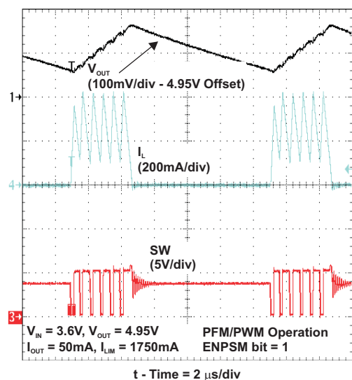
Figure 32. PFM OPERATION
