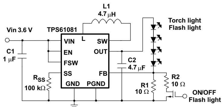
50 mA Torch Light and 100 mA Flash Light
