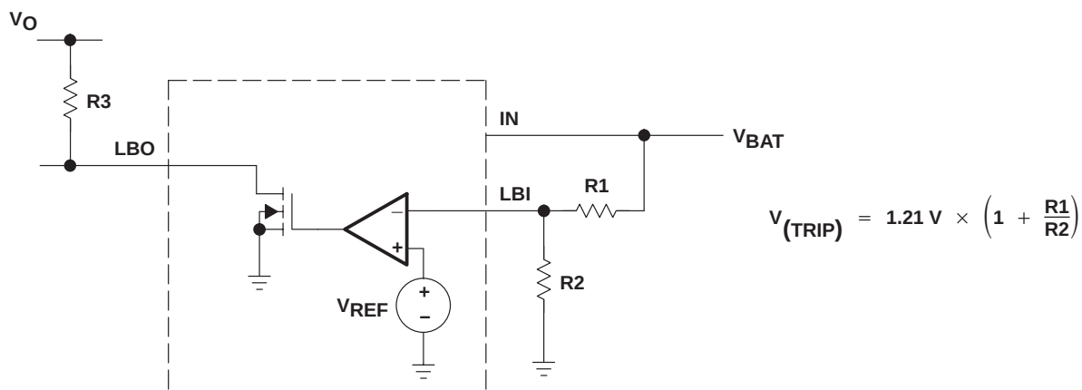
Figure 1. Programming of the Low-Battery Comparator Trip Voltage
