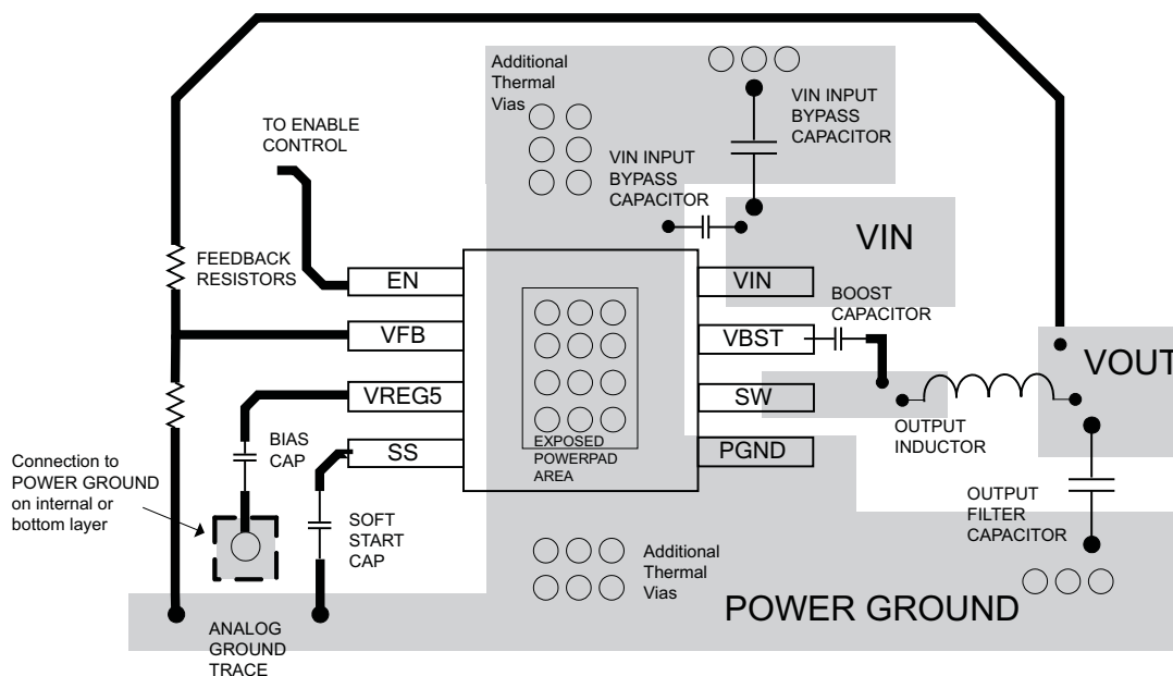
Figure 15. TPS54427 Layout
