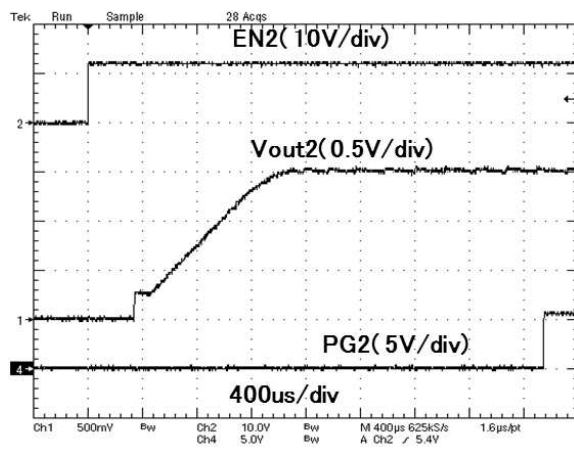
Figure 11. VO2=1.5V, PG
