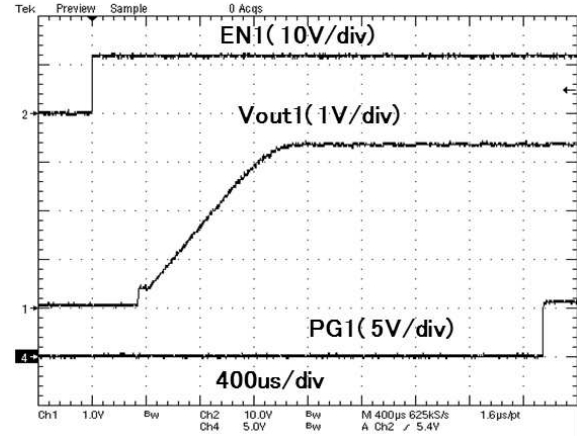
Figure 10. VO1=3.3V, PG
