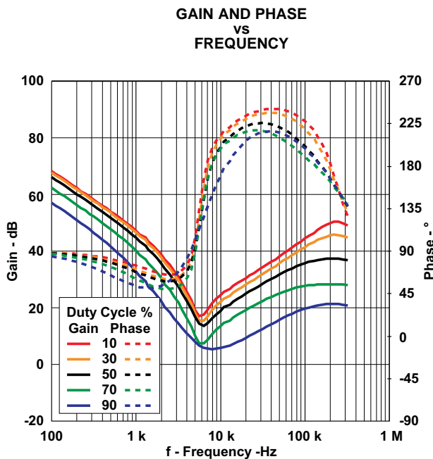
Figure 28. TPS54386 at 400-mA App Ripple Current
