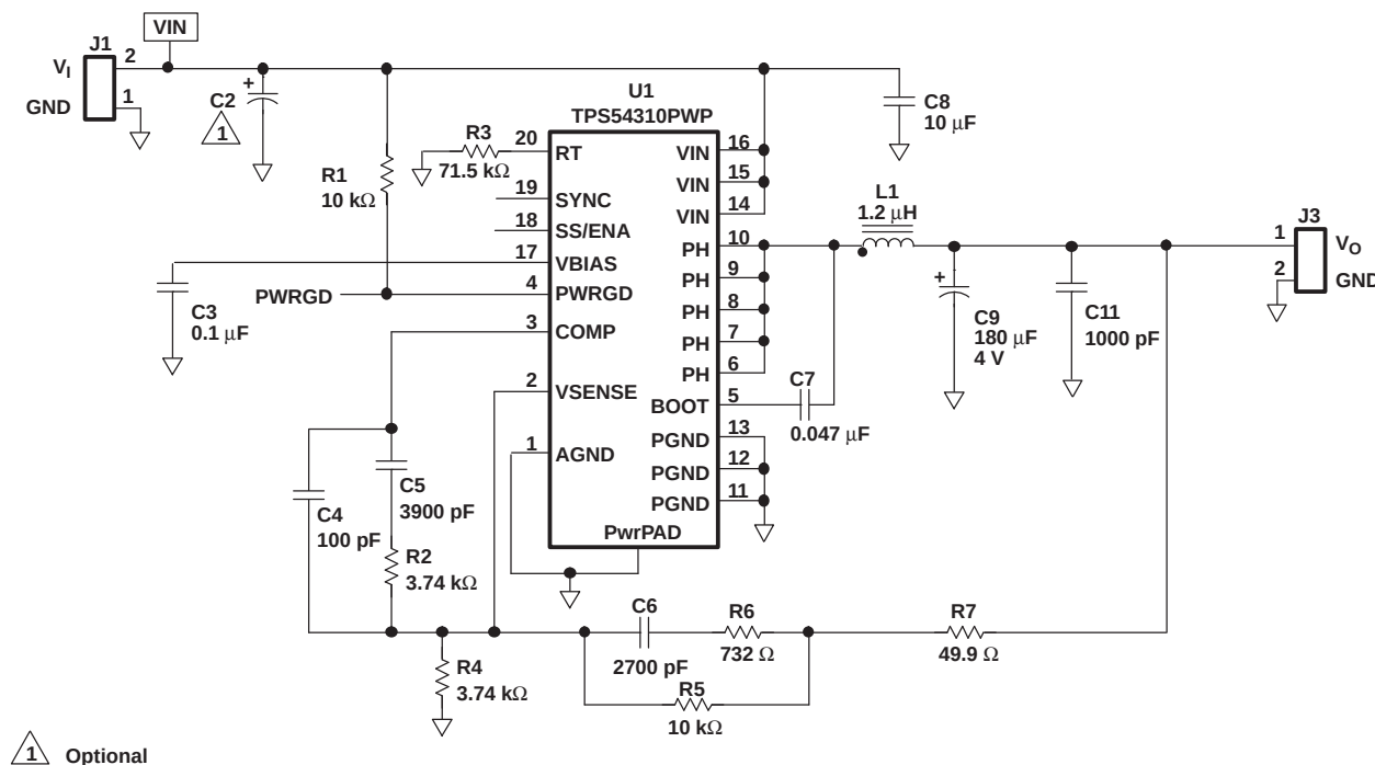
Figure 10. TPS54310 Schematic
