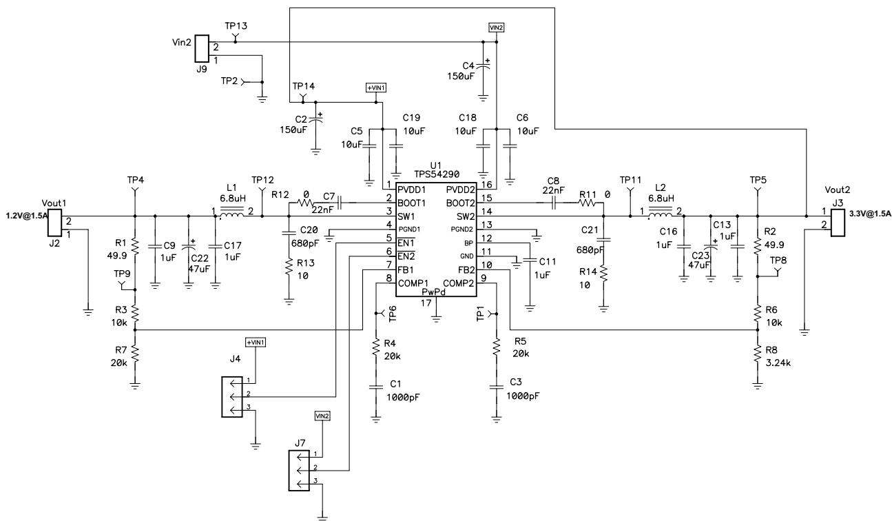
Figure 25. Cascading Operation
