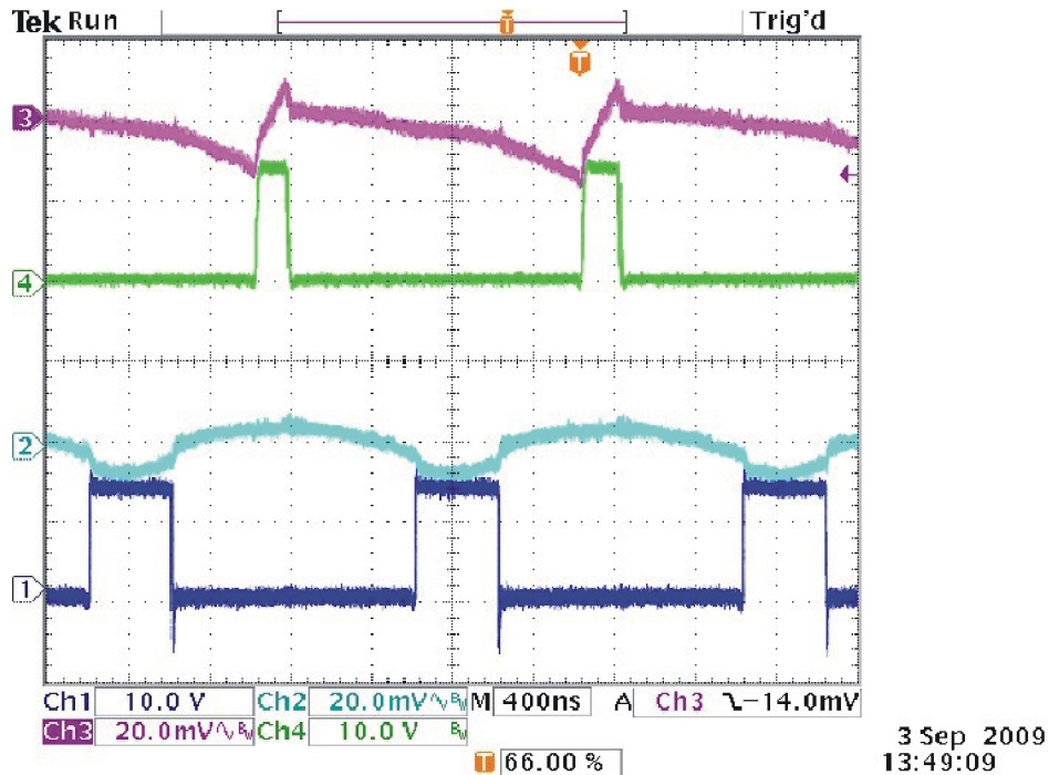
Figure 22. TPS54291 Design Example Switching Waveforms
