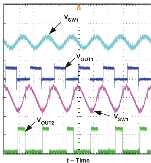
Figure 27. Output Ripple and SW Nodes
