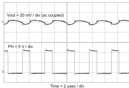
Figure 53. Output Ripple CCM
