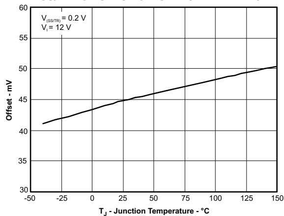
SS/TR TO VSENSE OFFSET vs TEMPERATURE
