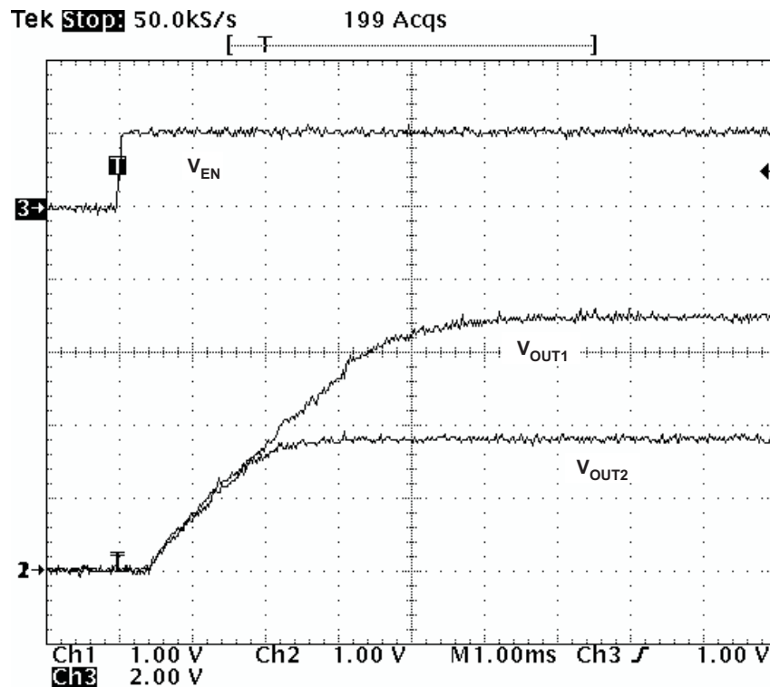
Figure 37. Simultaneous Start-Up
