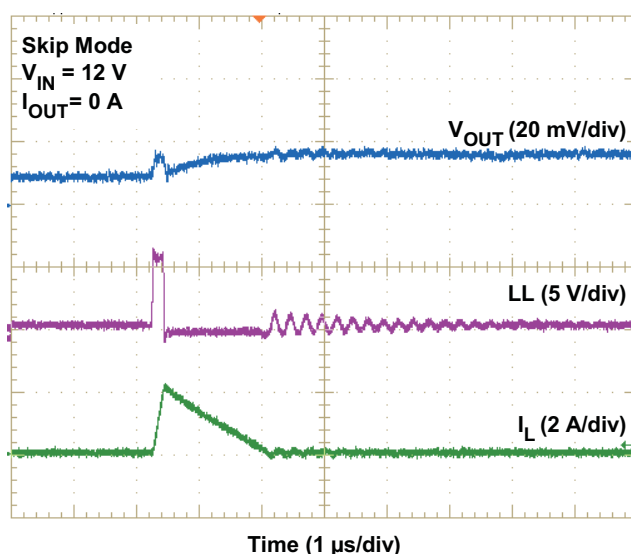
Figure 24. 1.1-V Output Skip Mode Steady-State Operation
