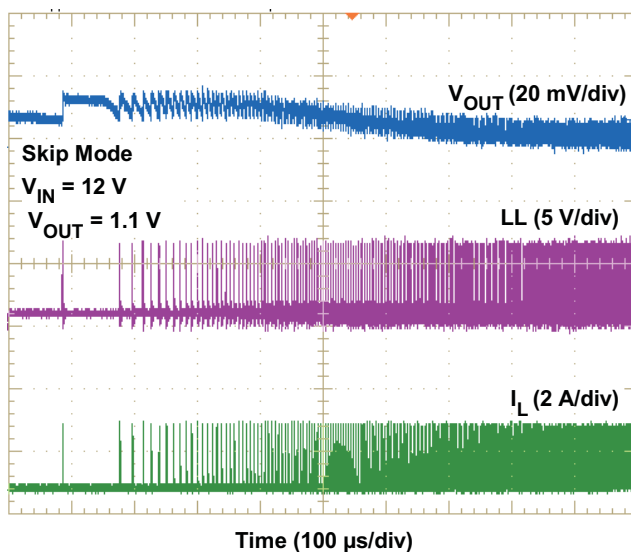
Figure 26. DCM to CCM Transition
