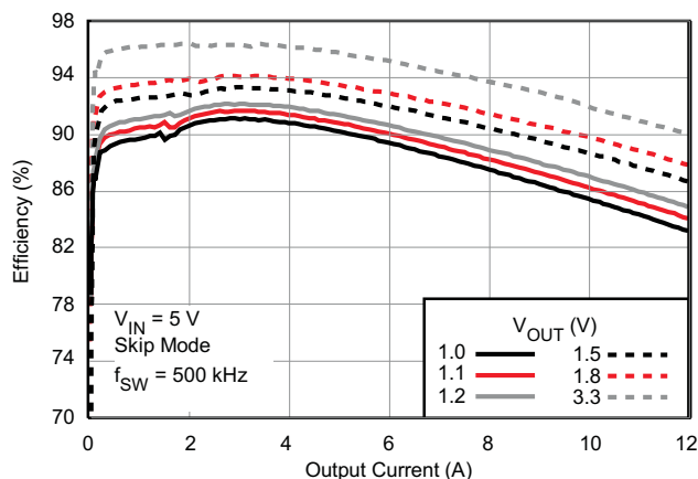
Figure 18. Efficiency vs Output Current, Inductor: HCB1175-501
