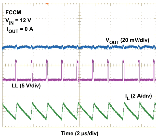
Figure 23. 1.1-V Output FCCM Steady-State Operation
