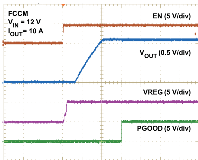
Figure 19. Start-Up
