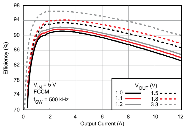
Figure 17. Efficiency vs Output Current, Inductor: HCB1175-501
