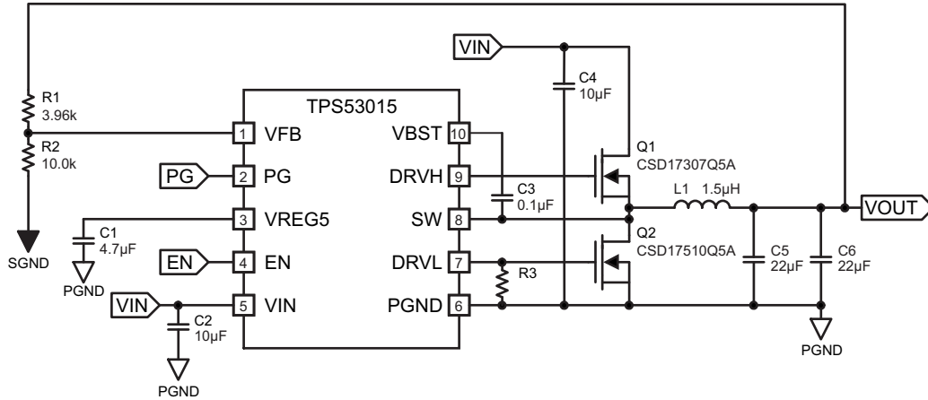
Figure 18. Application Schematic
