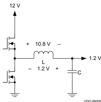
Figure 28. Synchronous Converter
