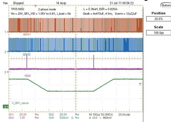
Figure 31. Dynamic VID: V_{IN} = 20V , SetVIDSlow = 0.6V, SetVIDSlow = 1.05V
