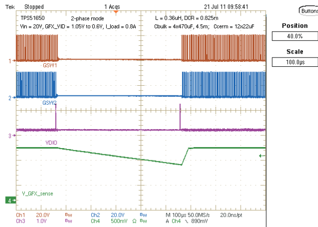
Figure 33. Dynamic VID: V_{IN} = 20V , SetVIDDecay = 0.6V, SetVIDFast 1.05V
