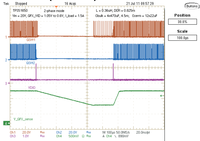
Figure 32. Dynamic VID: V_{IN} = 20V , SetVIDDecay = 0.6V, SetVIDFast = 1.05V
