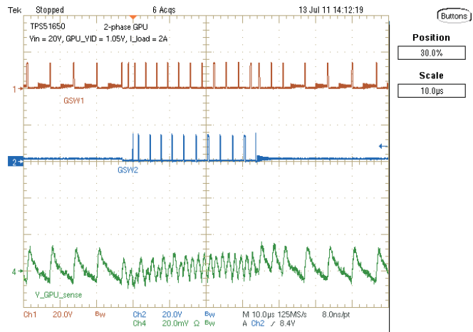
Figure 34. PS Change: V_{IN} = 20V , PS0 to PS1 Toggle
