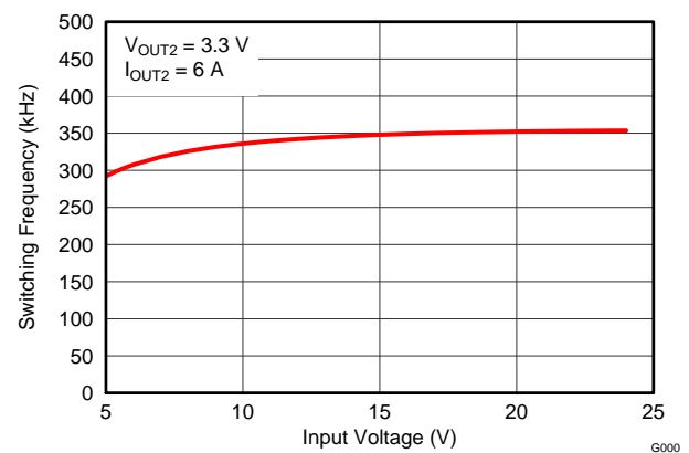
Figure 22. Switching Frequency vs. Input Voltage
