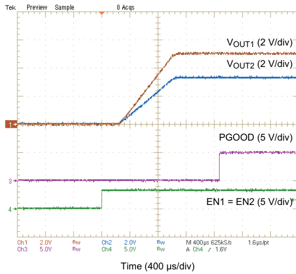
Figure 17. Start-Up
