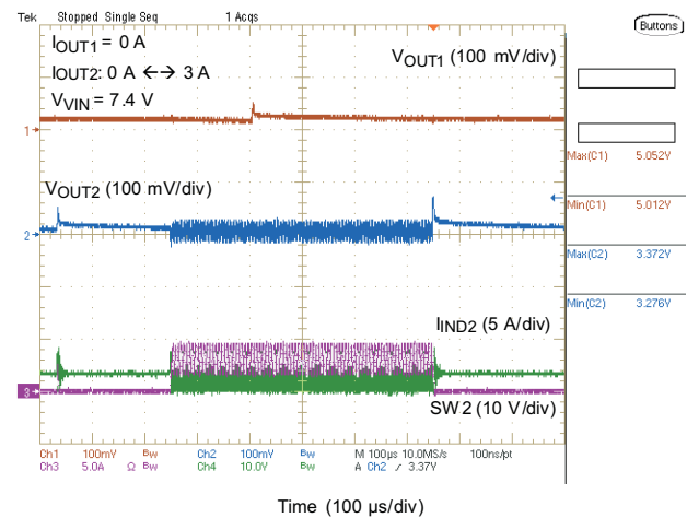
Figure 20. 3.3-V Load Transient
