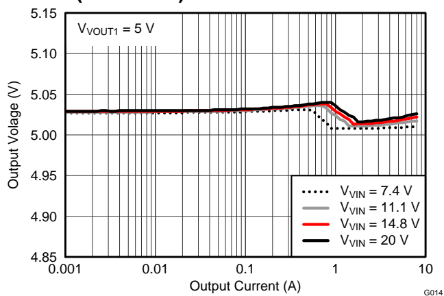
Figure 12. Load Regulation
