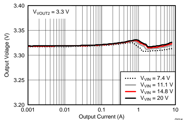
Figure 14. Load Regulation
