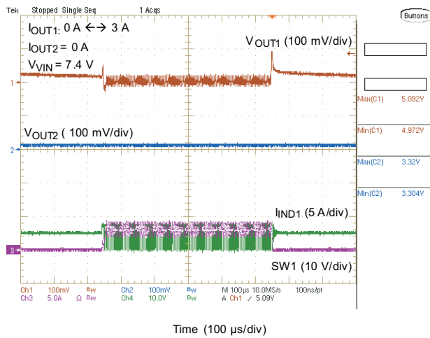
Figure 19. 5-V Load Transient
