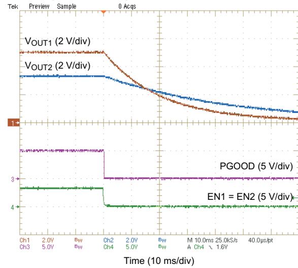
Figure 18. Output Discharge
