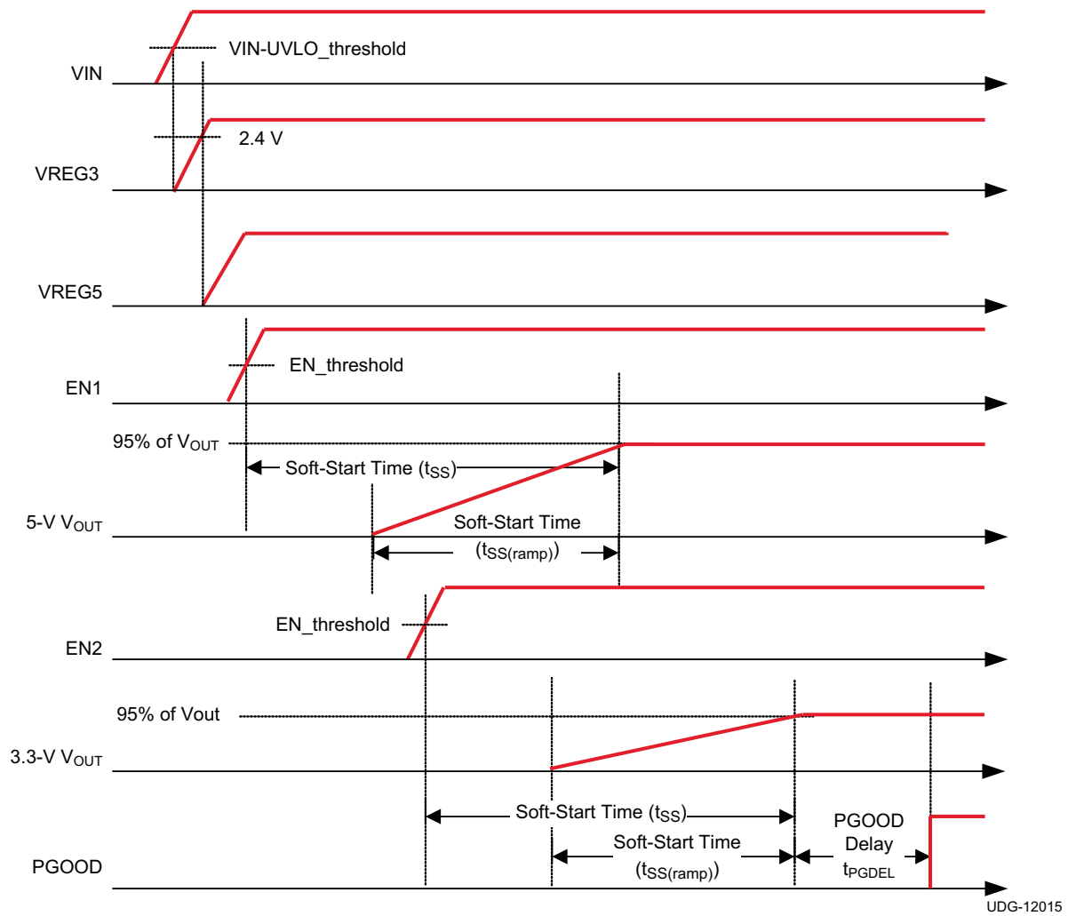
Figure 3. TPS51275C Timing
