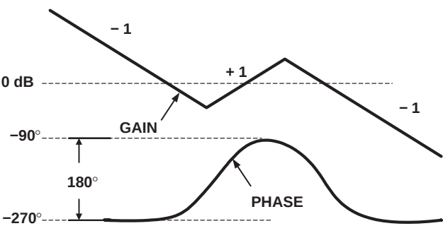
Figure 8. Type III Compensation Gain and Phase
