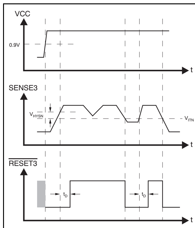
Figure 27. SVS-3 Timing Diagram
