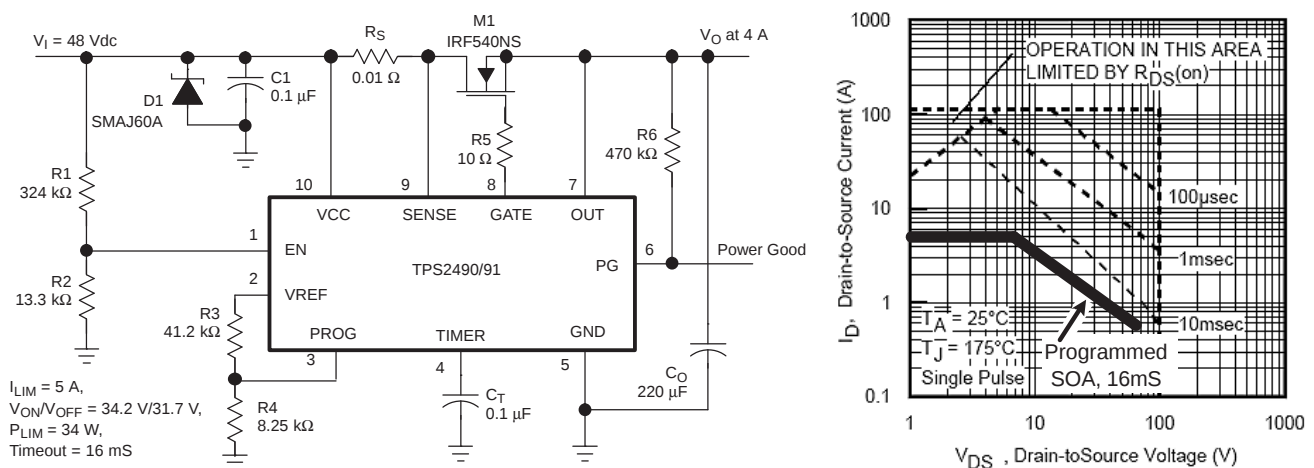
Figure 1. Typical Application and Corresponding SOA
