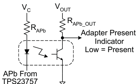
Figure 28. APb Interface
