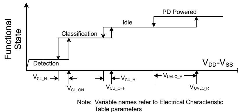
Figure 19. Threshold Voltages
