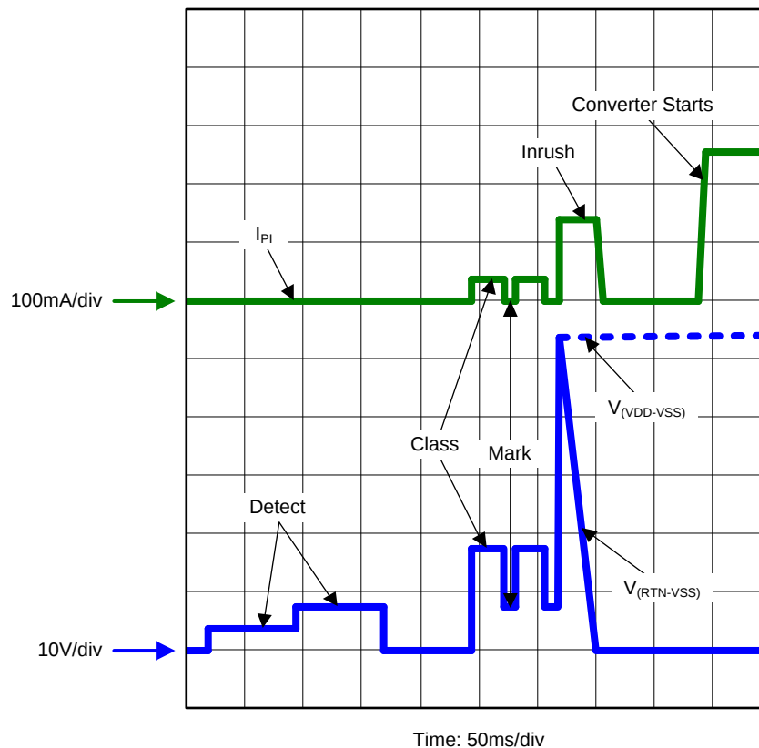
Figure 22. Startup
