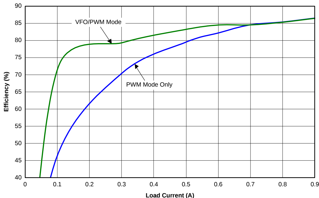
Figure 26. TPS23751 and TPS23752 Light Load Efficiency versus Mode
