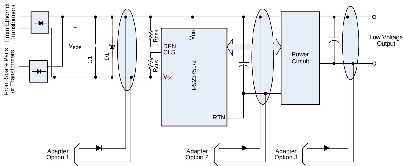
Figure 28. ORing Configurations
