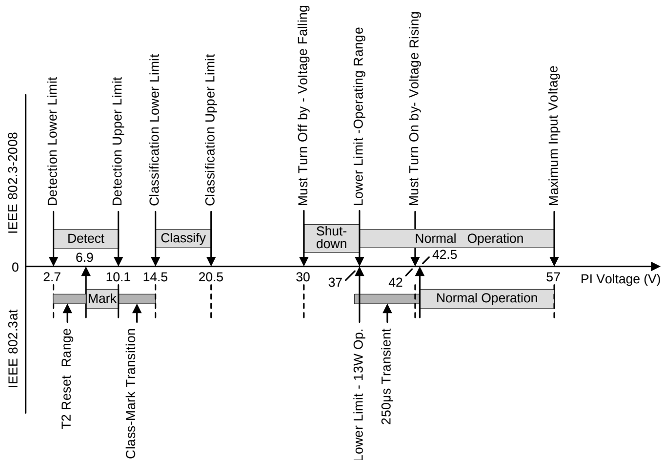
Figure 20. Threshold Voltages
