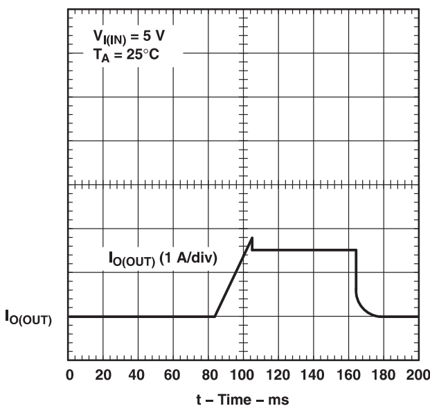
Figure 9. TPS2012A, Ramped Load on Enabled Device
