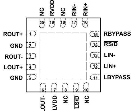
20-PIN QFN (RGW) PACKAGE (TOP VIEW)
