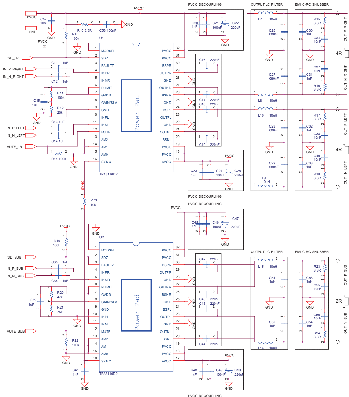
Figure 27. Schematic
