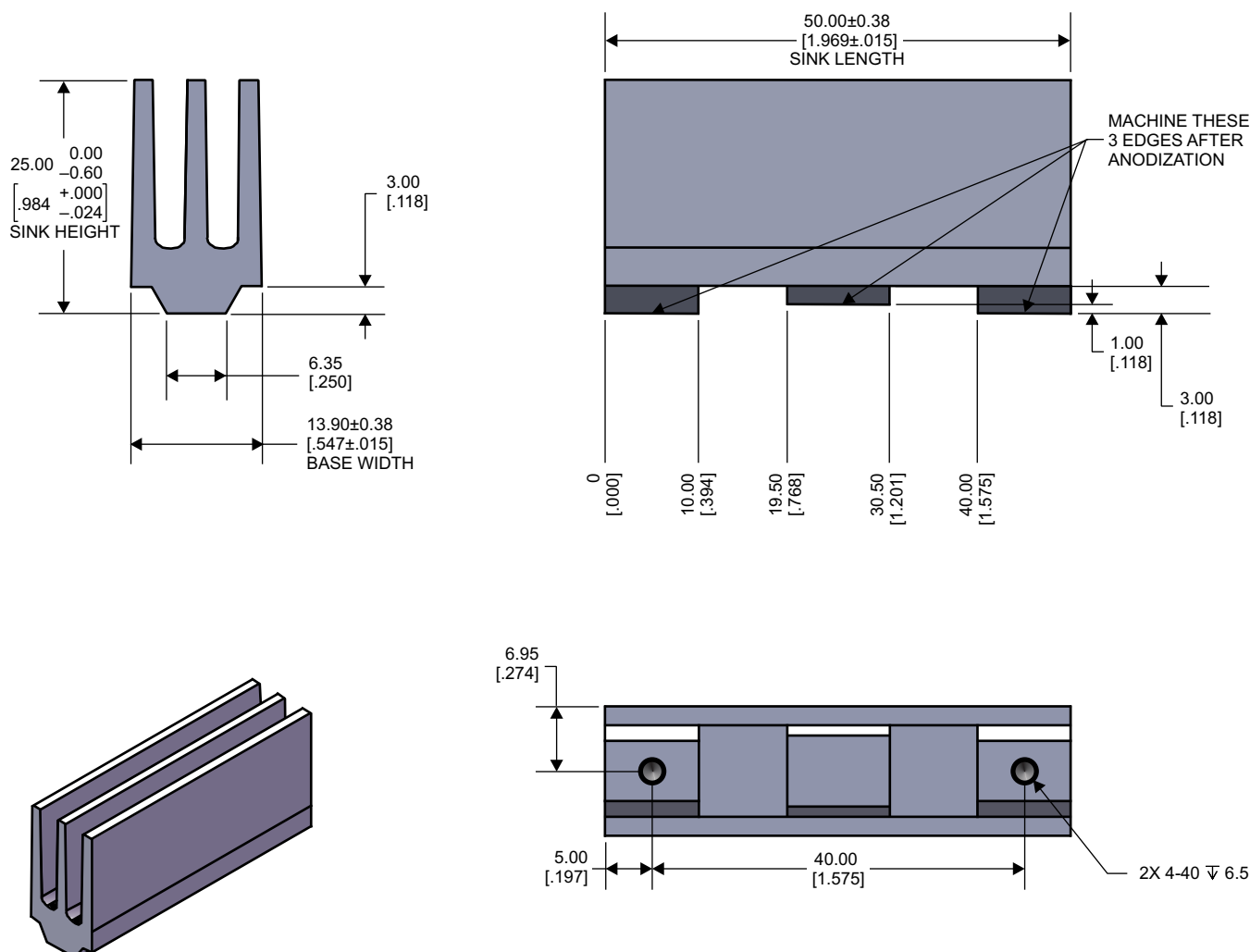
Figure 35. EVM Heatsink
