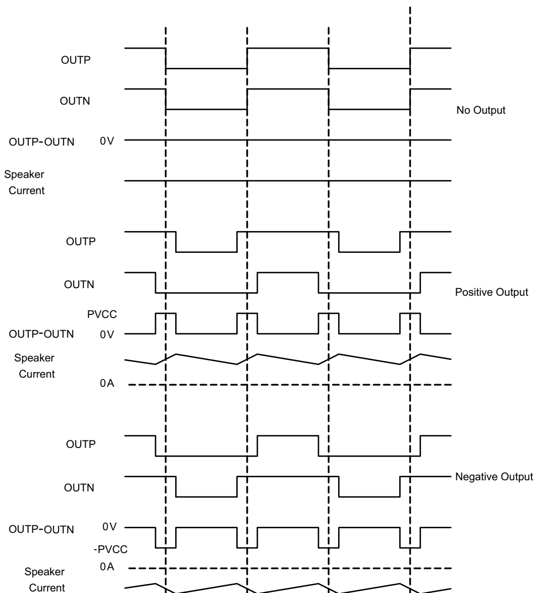
Figure 31. BD Mode Modulation
