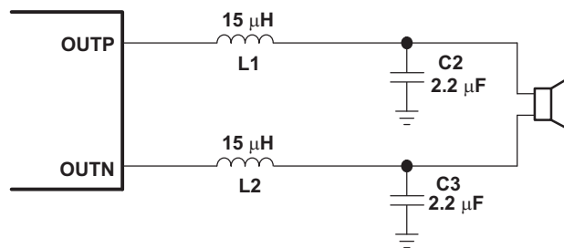
Figure 20. Typical LC Output Filter, Cutoff Frequency of 27 kHz, Speaker Impedance = 4 Ω
