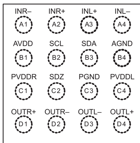
YZH (WCSP) PACKAGE (Top View)
