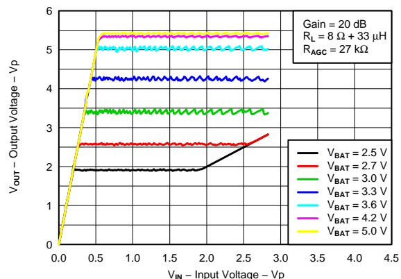
Figure 4. PEAK OUTPUT VOLTAGE vs PEAK INPUT VOLTAGE
