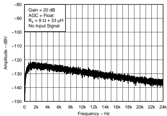
Figure 2. A-WEIGHTED OUTPUT NOISE vs FREQUENCY
