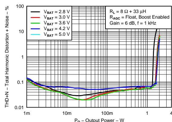
Figure 6. TOTAL HARMONIC DISTORTION + NOISE vs OUTPUT POWER
