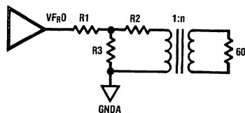
FIGURE 3. Receive Gain Adjustment
