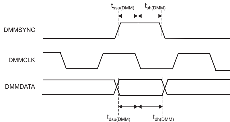
Figure 4-28. DMMDATA Timing
