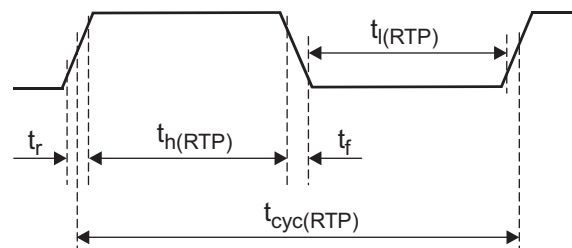
Figure 4-24. RTPCLK Timing
