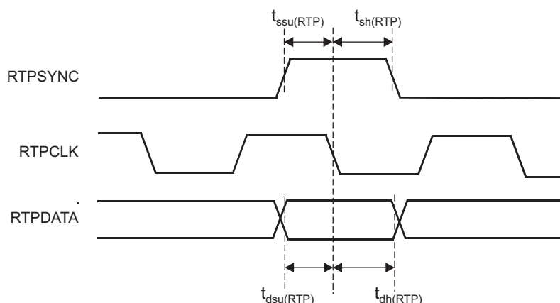
Figure 4-25. RTPDATA Timing
