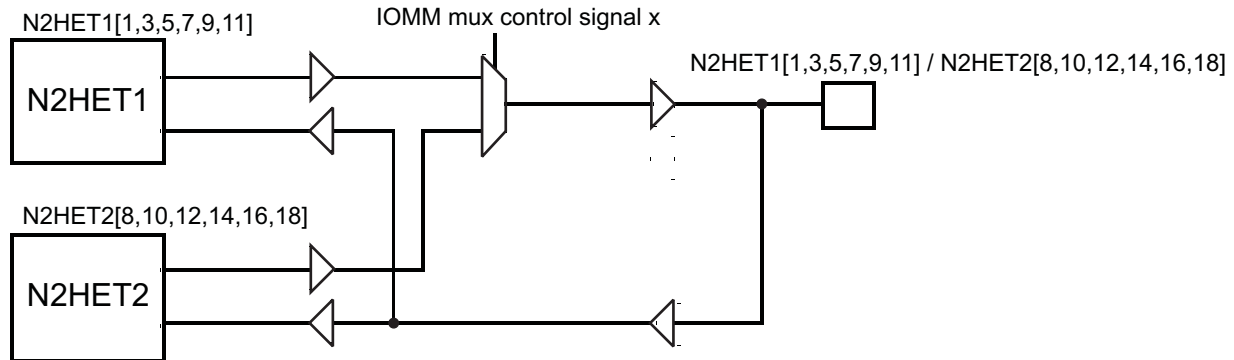
Figure 5-7. N2HET Monitoring
