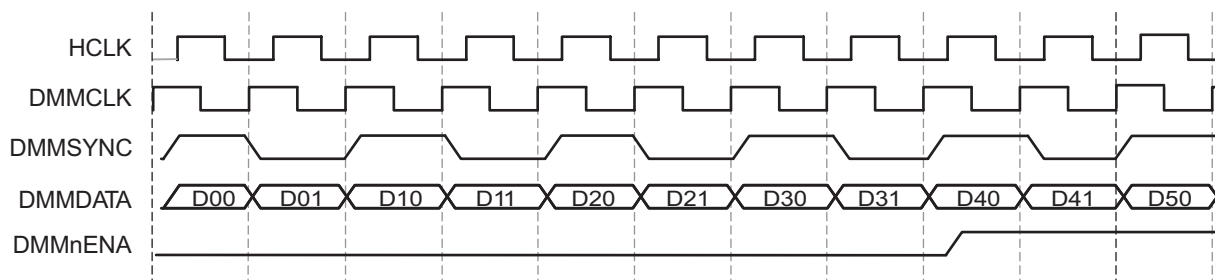
Figure 4-29. DMMnENA Timing
