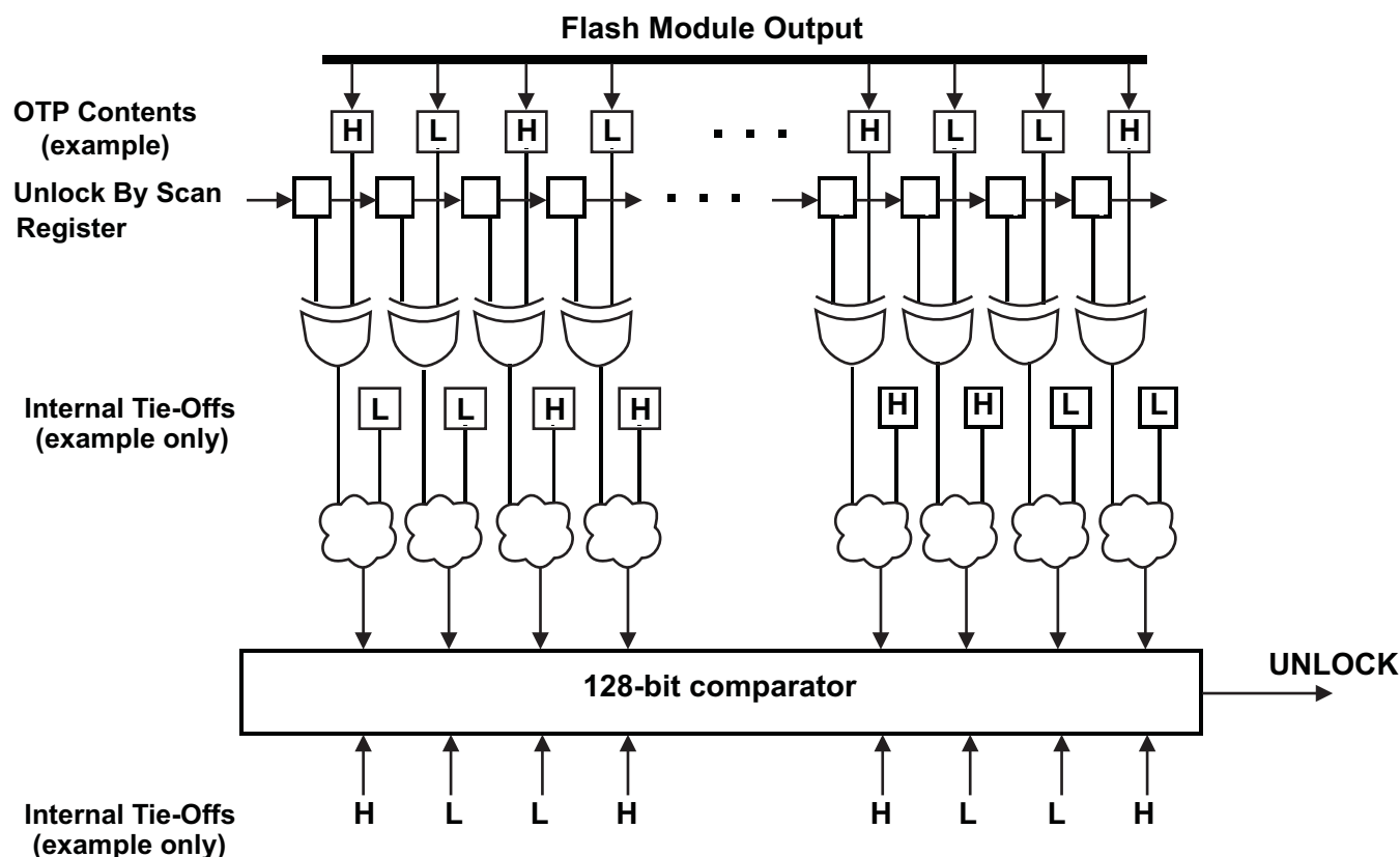
Figure 4-21. AJSM Unlock
