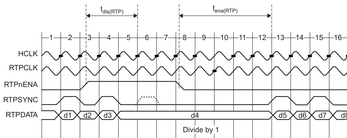
Figure 4-26. RTPnENA timing
