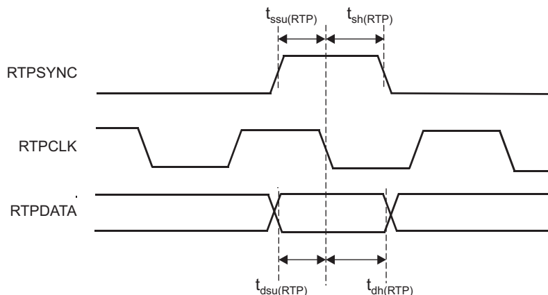
Figure 4-25. RTPDATA Timing
