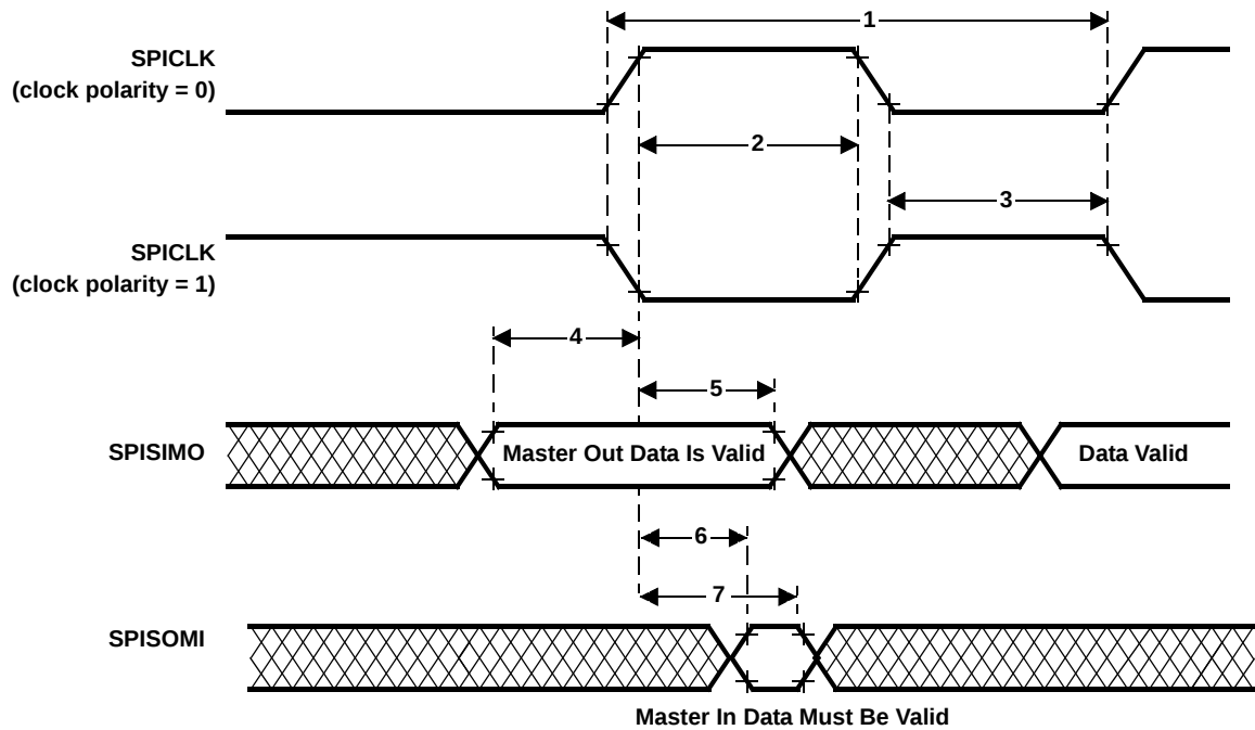
Figure 15. MibSPI Master Mode External Timing (CLOCK PHASE = 1)
