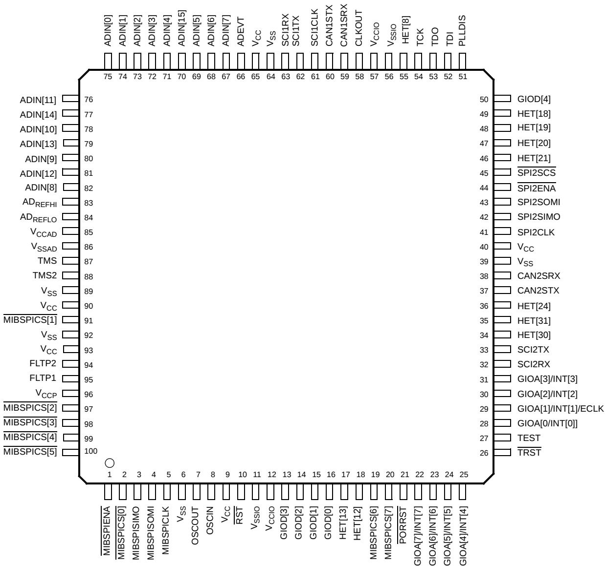
TMS470R1VF448 100-PIN PZ PACKAGE (TOP VIEW)
