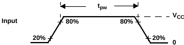
Figure 9. CMOS-Level Inputs
