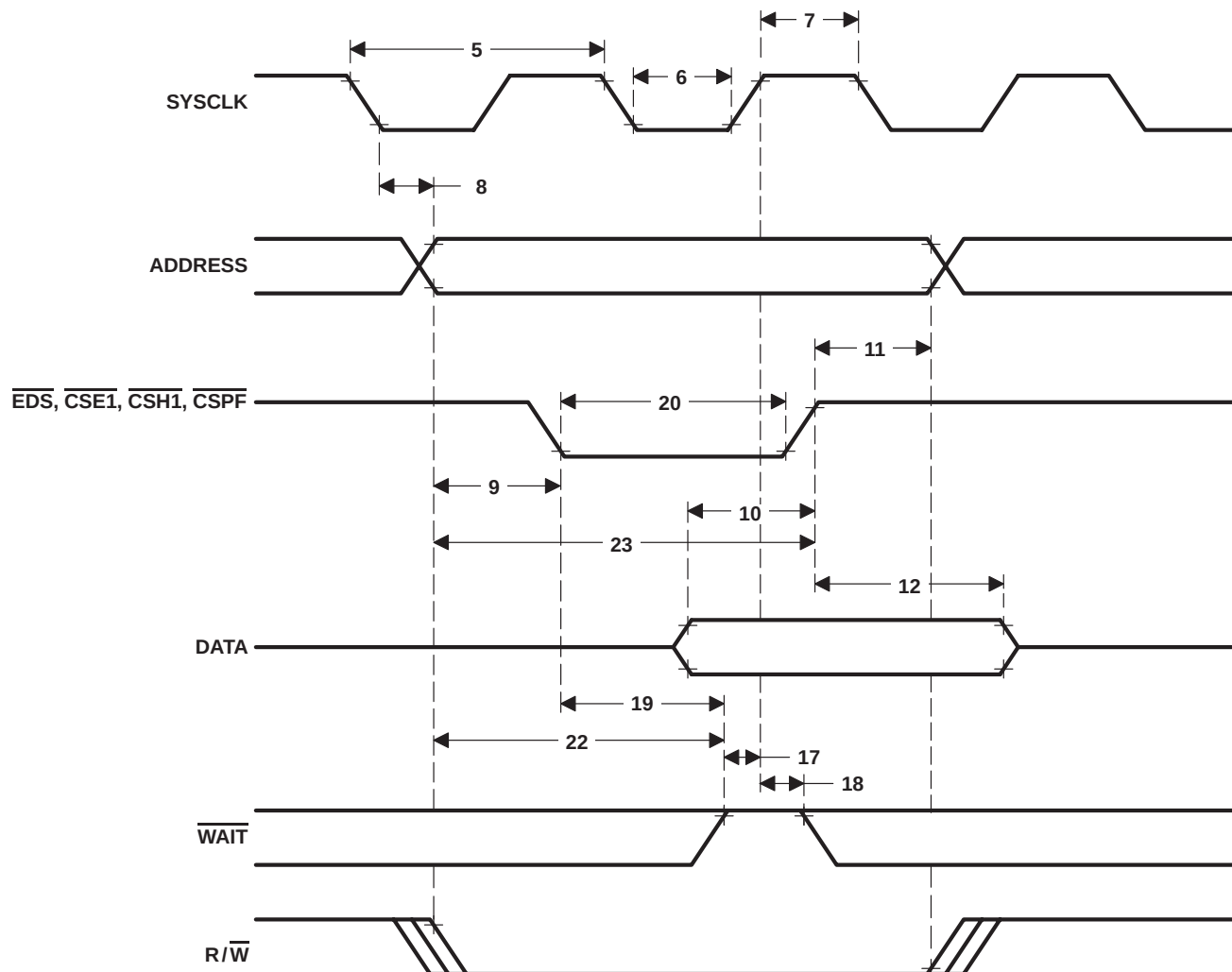
Figure 28. External-Write Timing
