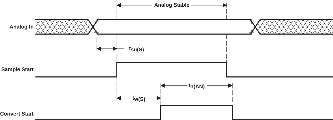
Figure 33. Analog Timing
