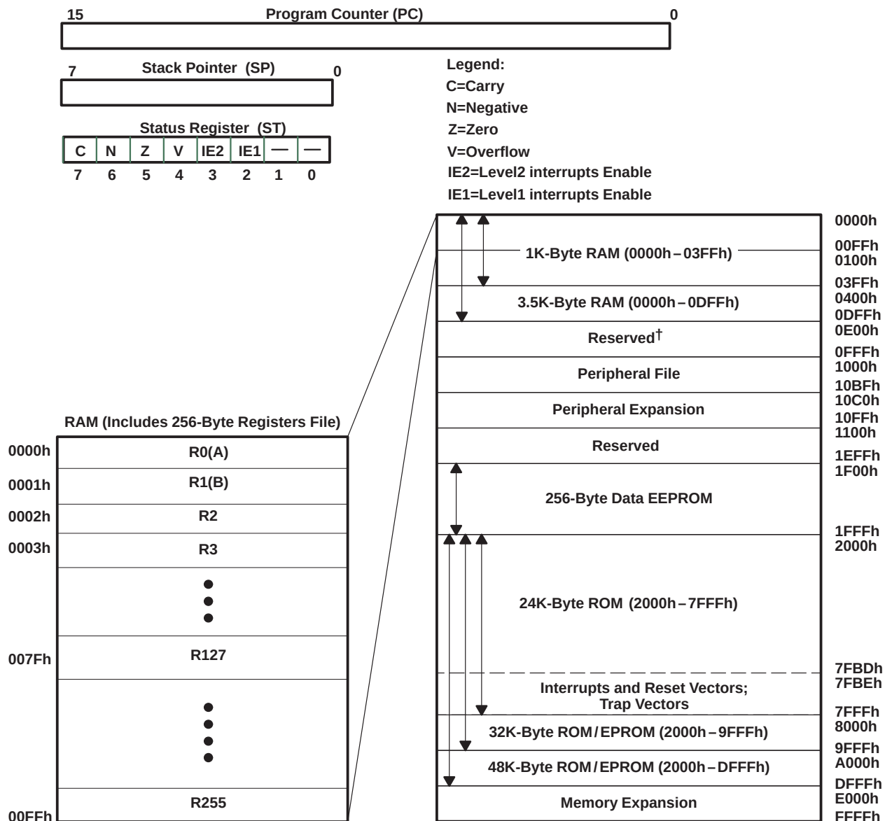
Figure 1. Programmer's Model
