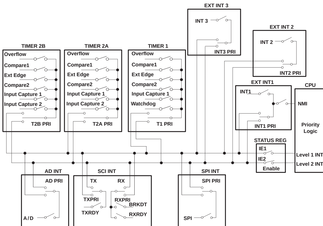
Figure 4. Interrupt Control
