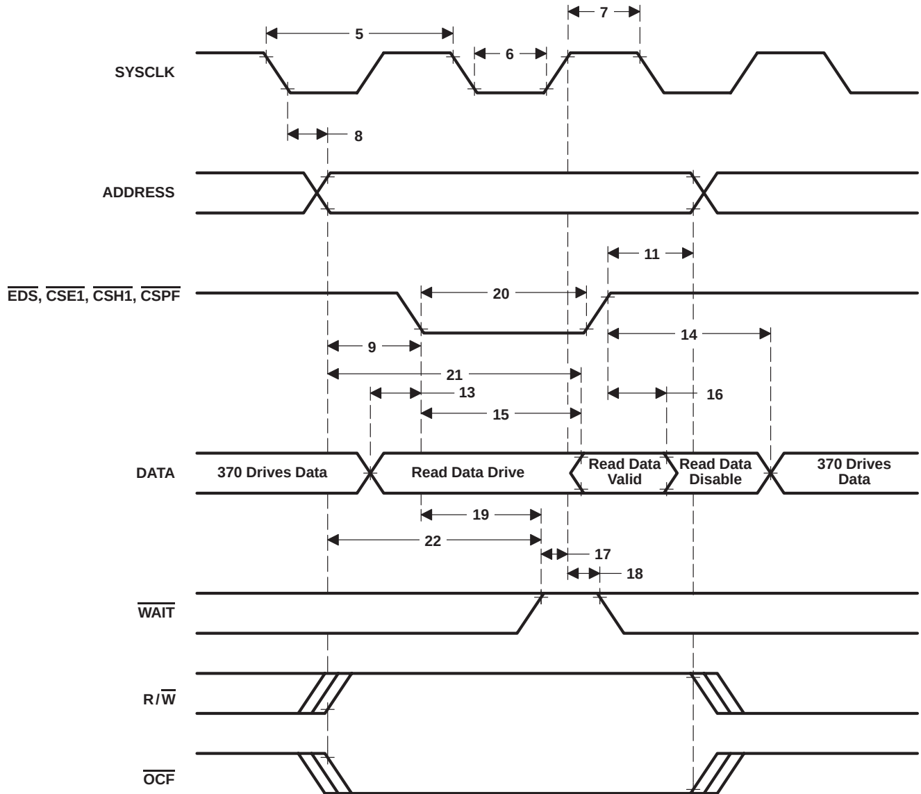
Figure 27. External-Read Timing
