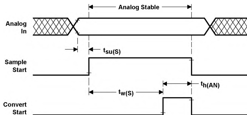
Figure 24. Analog Timing
