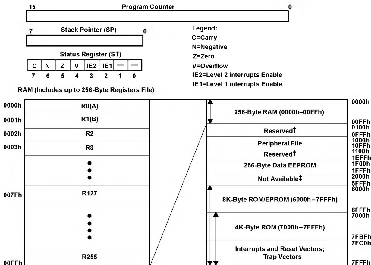
Figure 1. Programmer's Model
