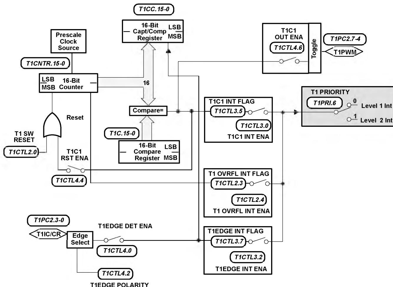
Figure 7. Capture/Compare Mode
