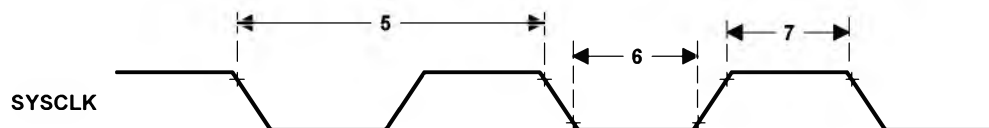
Figure 23. SYSCLK Timing
