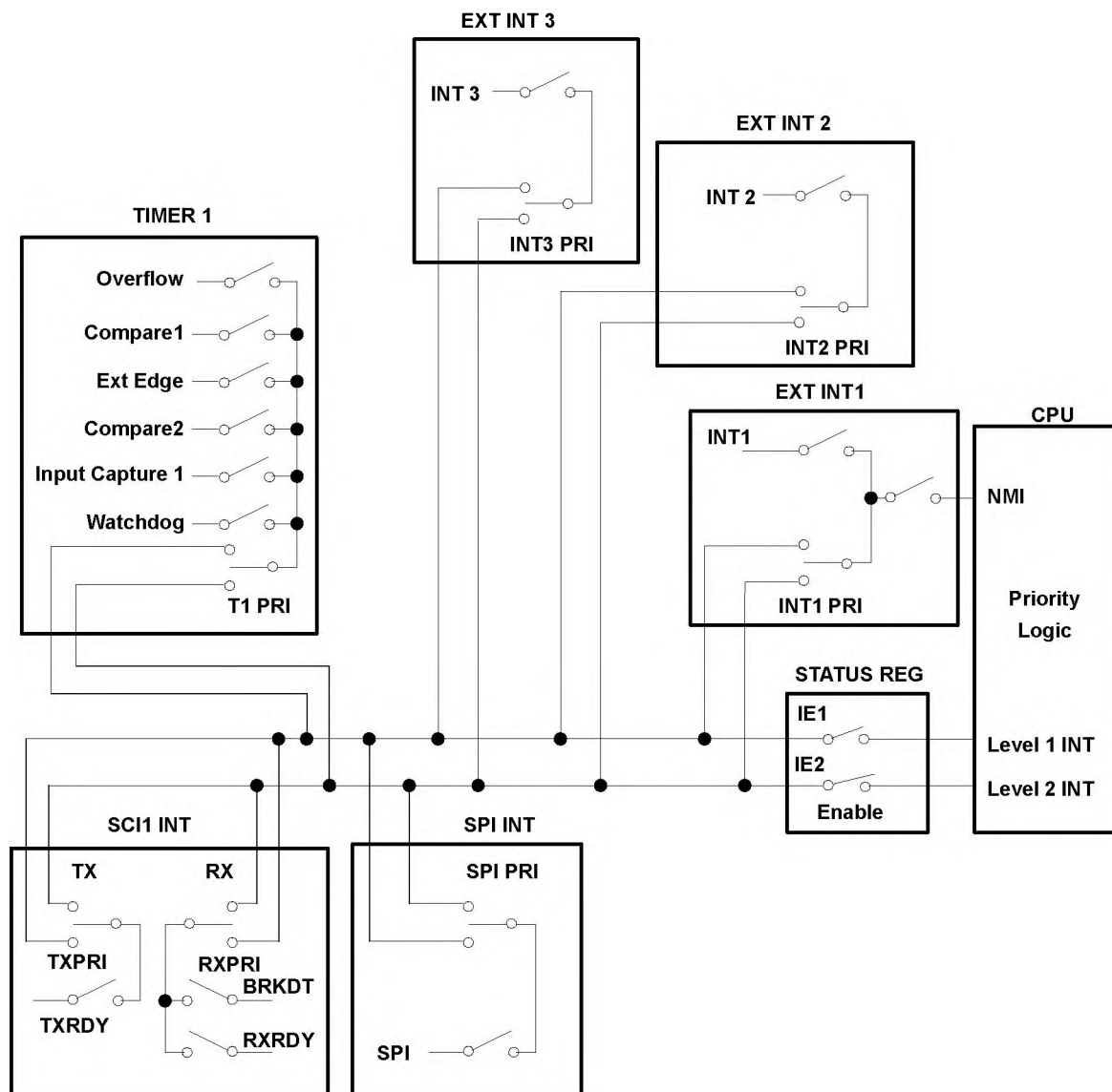
Figure 5. Interrupt Control
