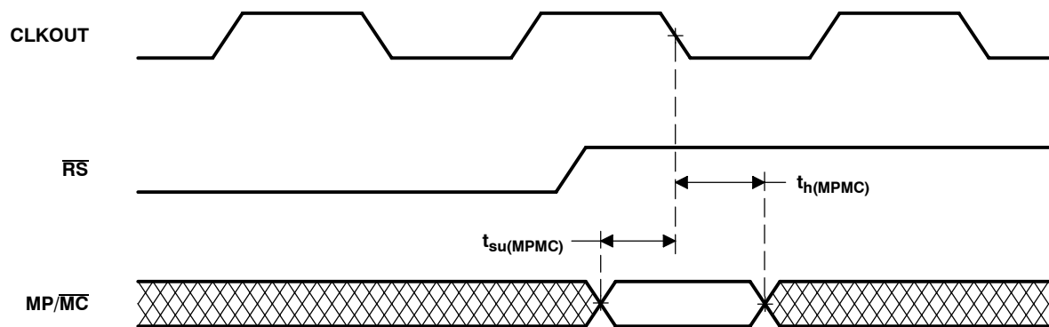
Figure 4-17. MP/MC Timing
