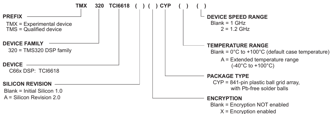
Figure 2-17 C66x™ DSP Device Nomenclature (including the TMS320TCI6618 DSP)
