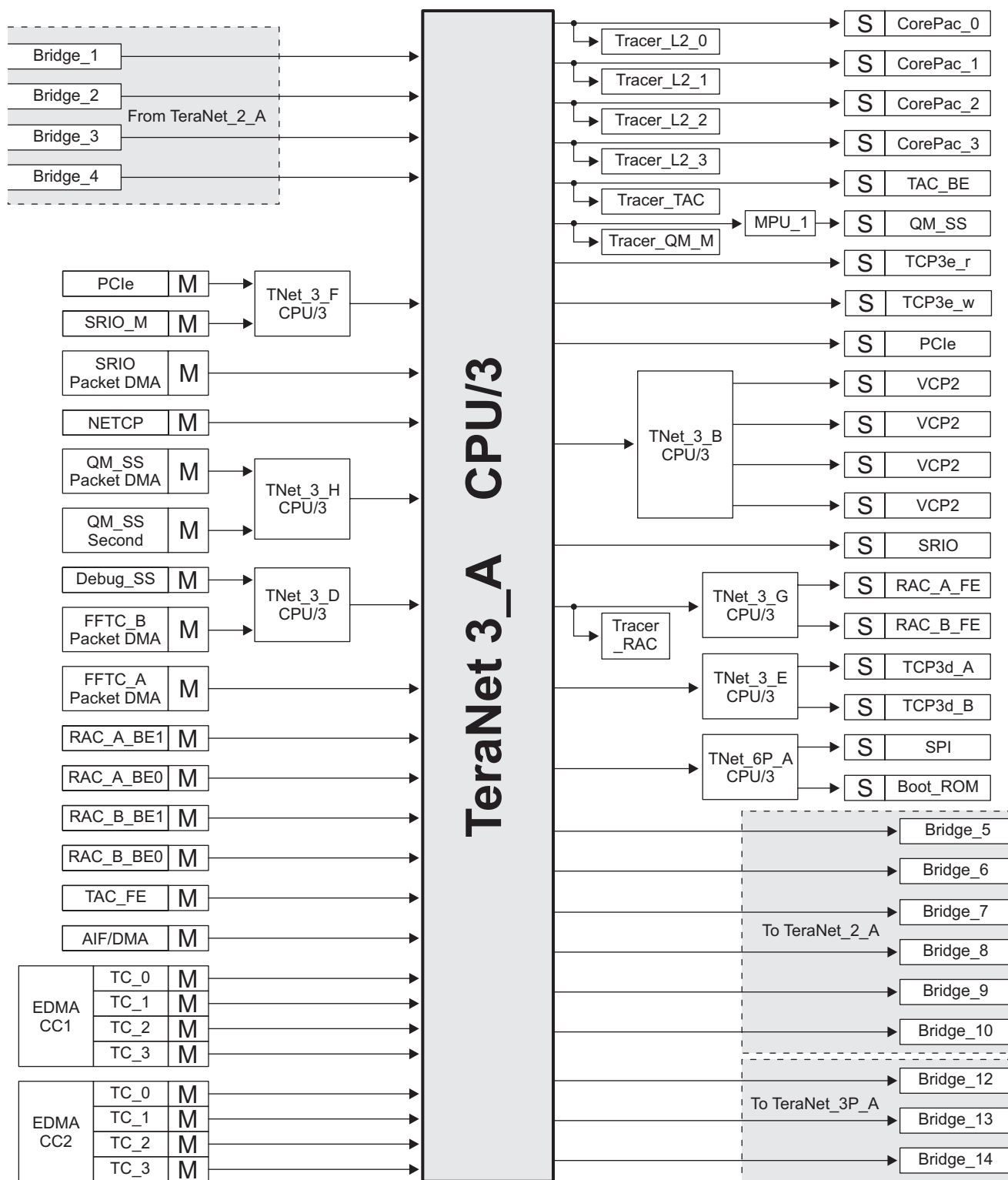
Figure 4-1 TeraNet 3A
