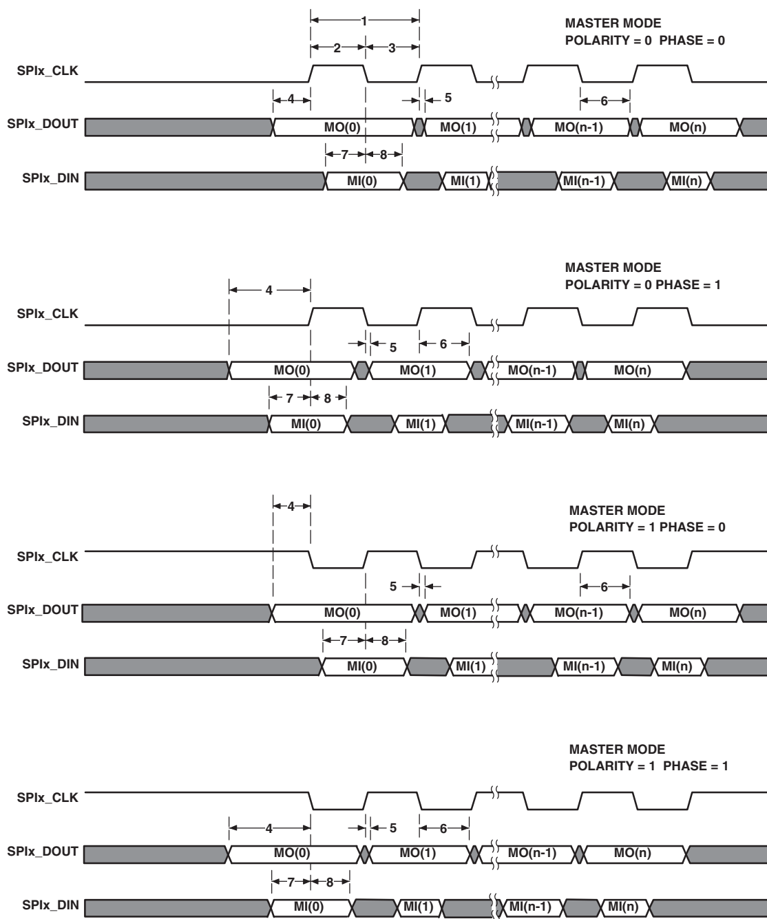
Figure 8-39 SPI Master Mode Timing Diagrams — Base Timings for 3-Pin Mode
