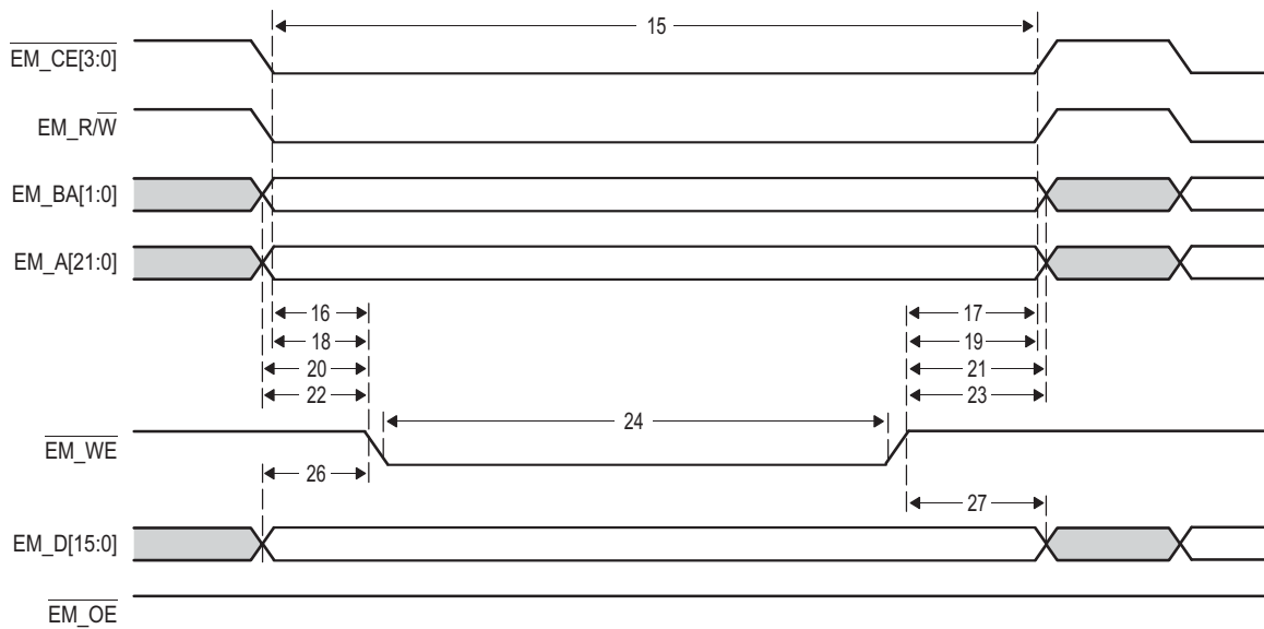
Figure 8-61 EMIF16 Asynchronous Memory Write Timing Diagram
