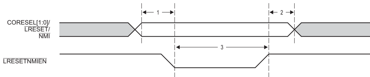
Figure 8-30 NMI and LRESET Timing
