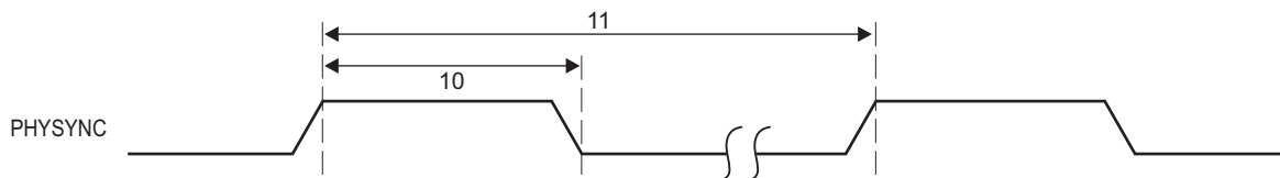
Figure 8-57 AIF2 Physical Layer Synchronization Pulse Timing
