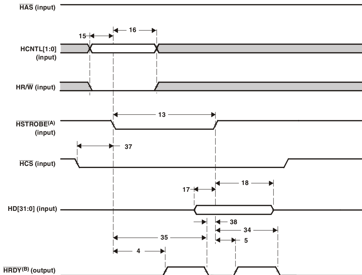
Figure 8-34 HPI32 Write Timing ( \overline{\text{HAS}} Not Used, Tied High)
