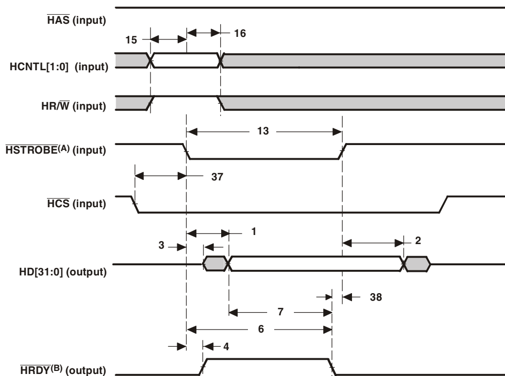
Figure 8-32 HPI32 Read Timing ( \overline{\text{HAS}} Not Used, Tied High)
