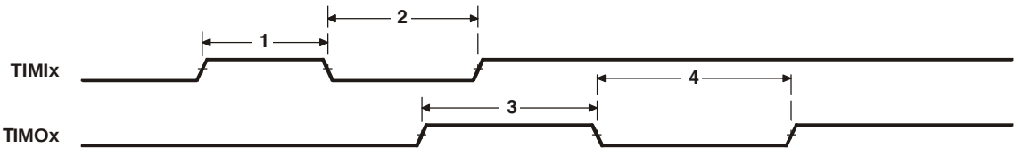
Figure 8-45 Timer Timing
