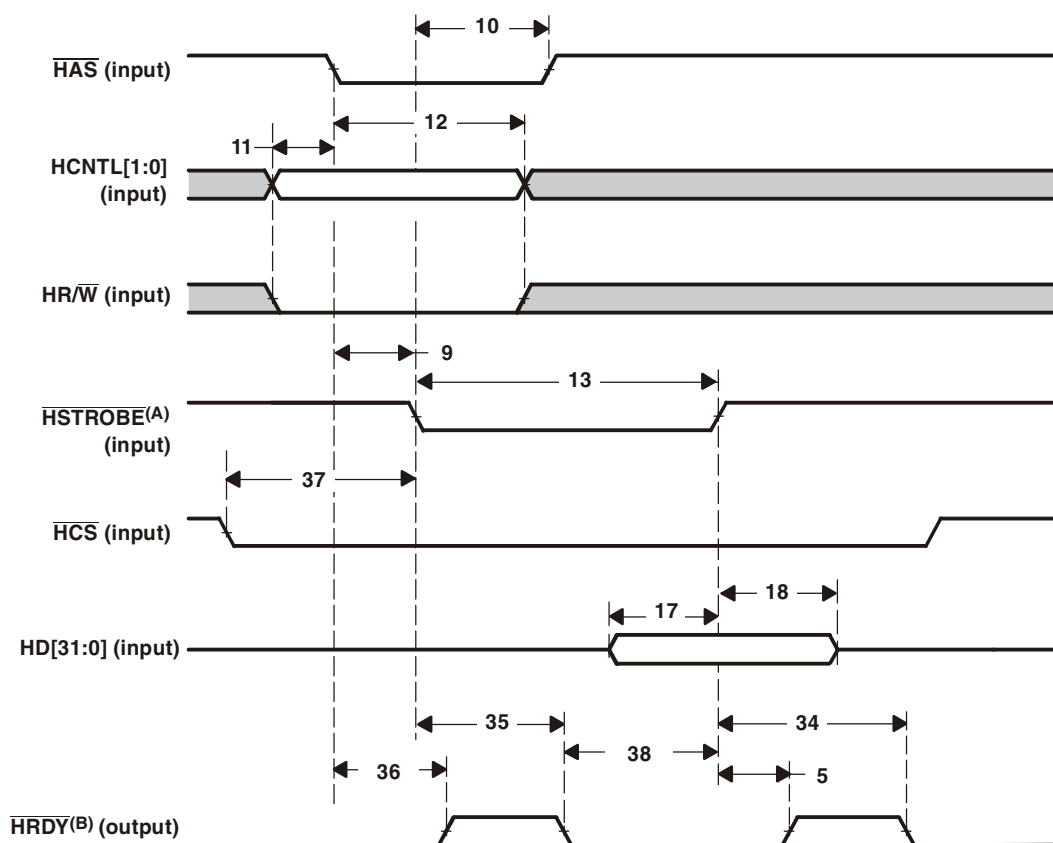
Figure 8-35 HPI32 Write Timing (HAS Used)
