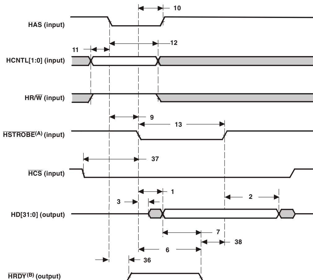
Figure 8-33 HPI32 Read Timing (HAS Used)
