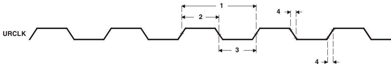
Figure 8-47 URCLK Timing
