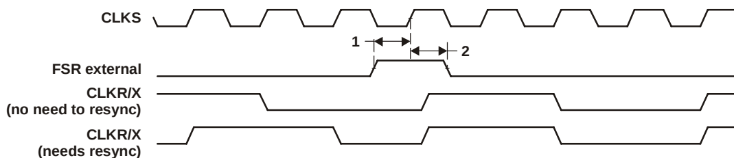
Figure 8-37 FSR Timing When GSYNC = 1
