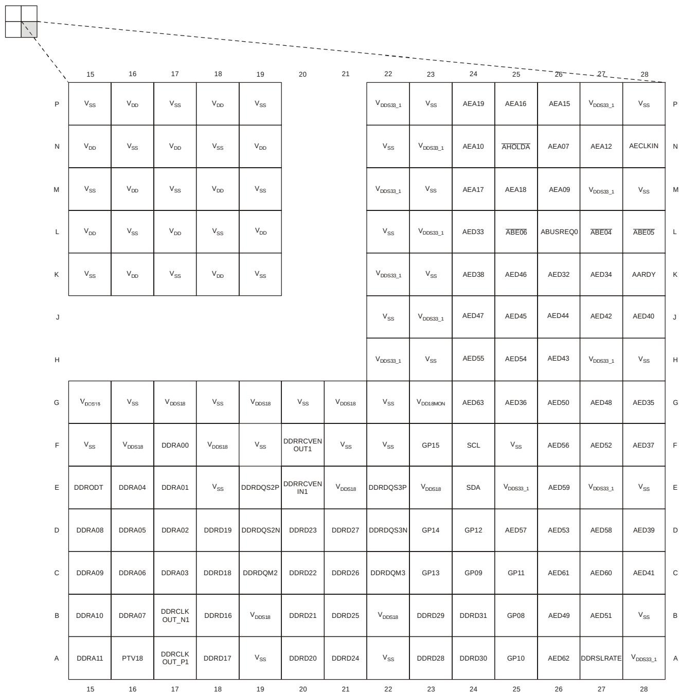
Figure 2-4 TMS320TCI6484 Pin Map (Bottom View) [Quadrant C]
