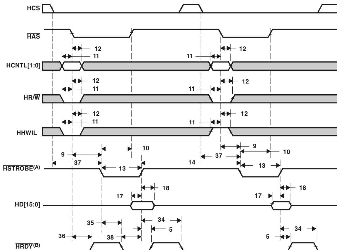
Figure 8-31 HPI16 Write Timing (HAS Used)
