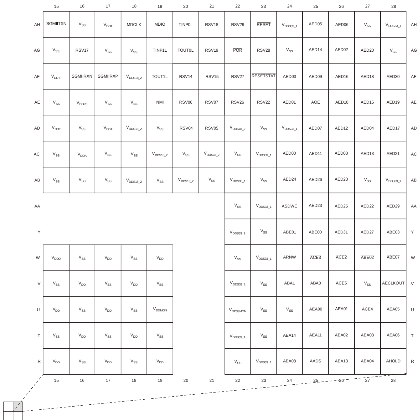
Figure 2-3 TMS320TCI6484 Pin Map (Bottom View) [Quadrant B]
