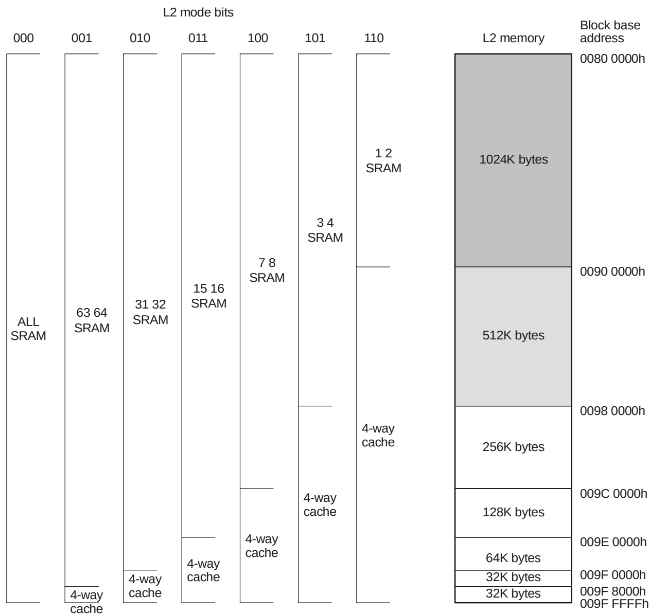
Figure 5-4 TMS320TCI6484 L2 Memory Configurations
