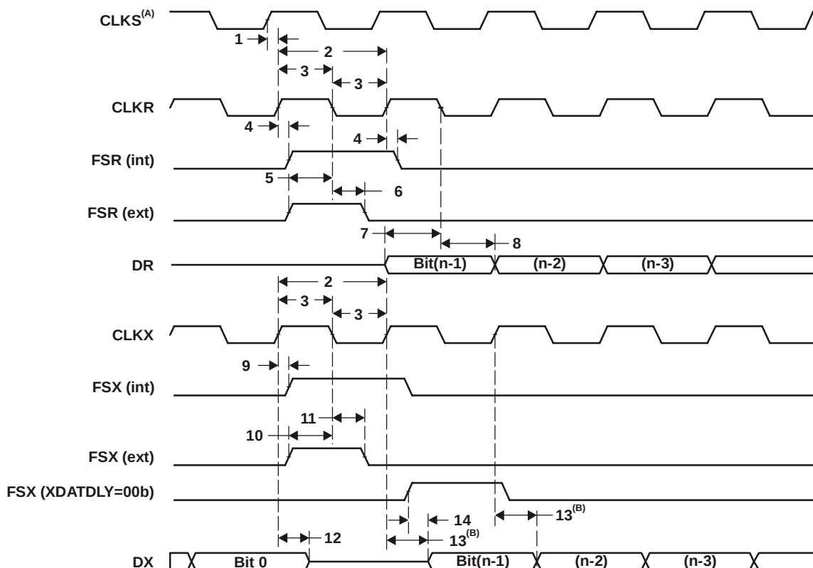
Figure 8-36 McBSP Timing
