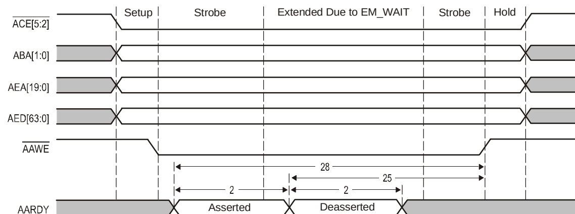
Figure 8-21 EMIFA EM_Wait Write Timing Requirements
