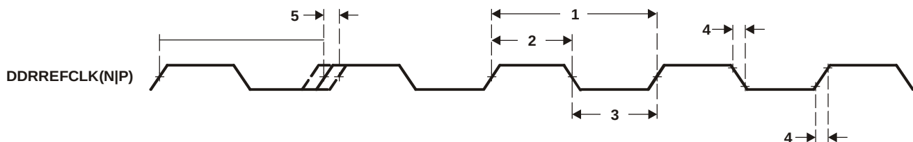
Figure 8-15 DDRREFCLK(N|P) Timing
