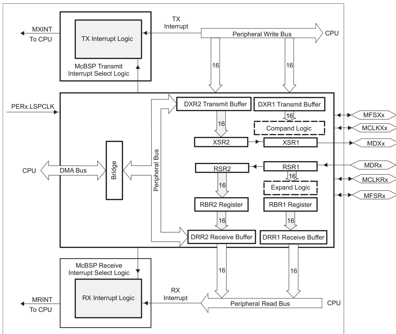
Figure 5-57. McBSP Block Diagram
