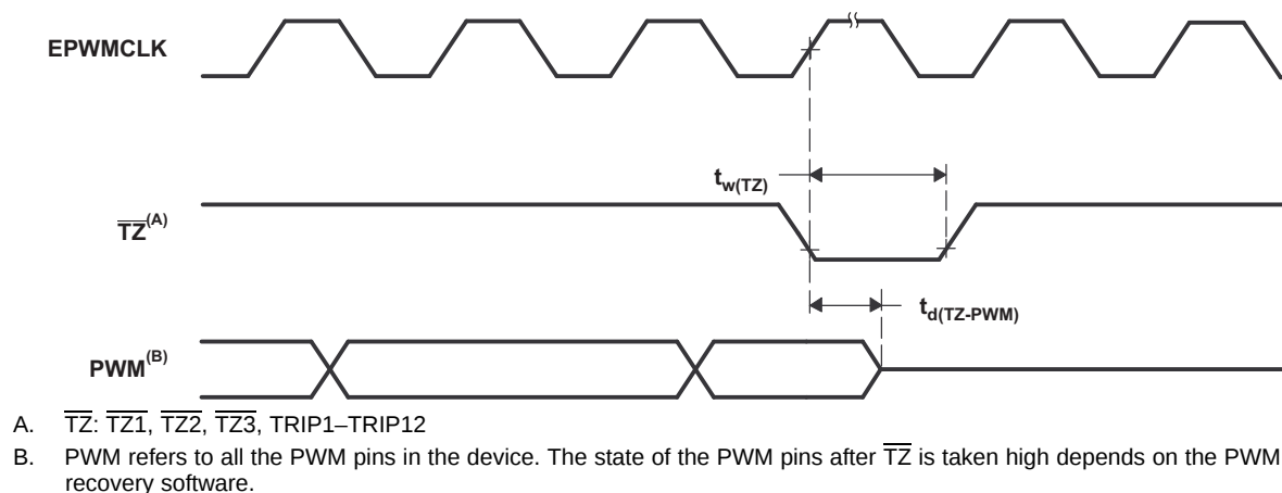
Figure 5-48. PWM Hi-Z Characteristics
