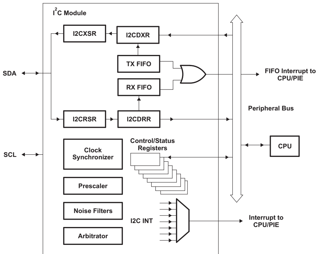
Figure 5-56. I2C Peripheral Module Interfaces
