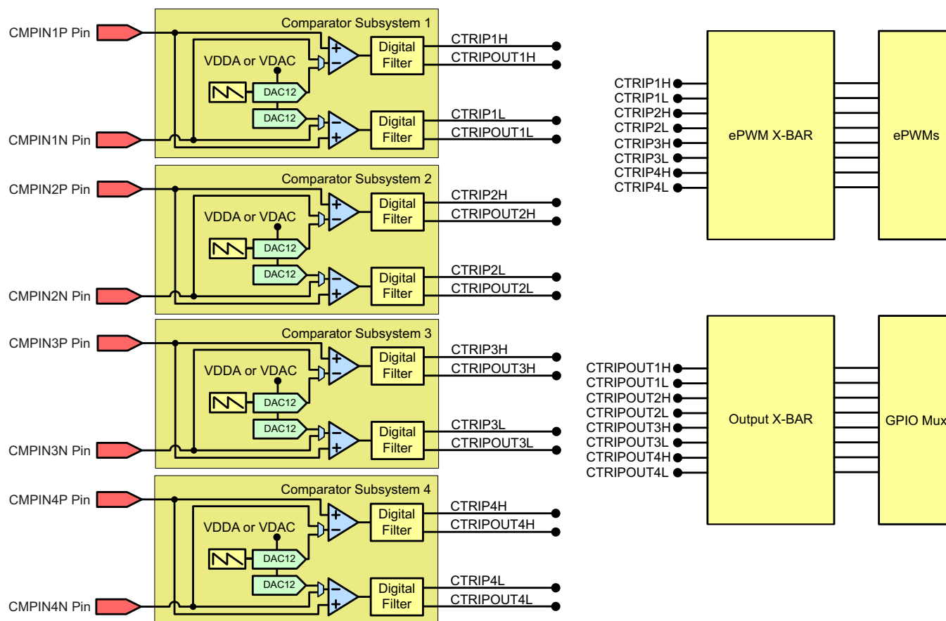
Figure 5-34. CMPSS Connectivity (100-Pin PZP)
