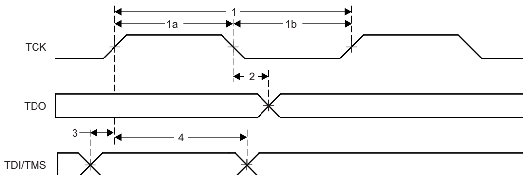
Figure 5-11. JTAG Timing
