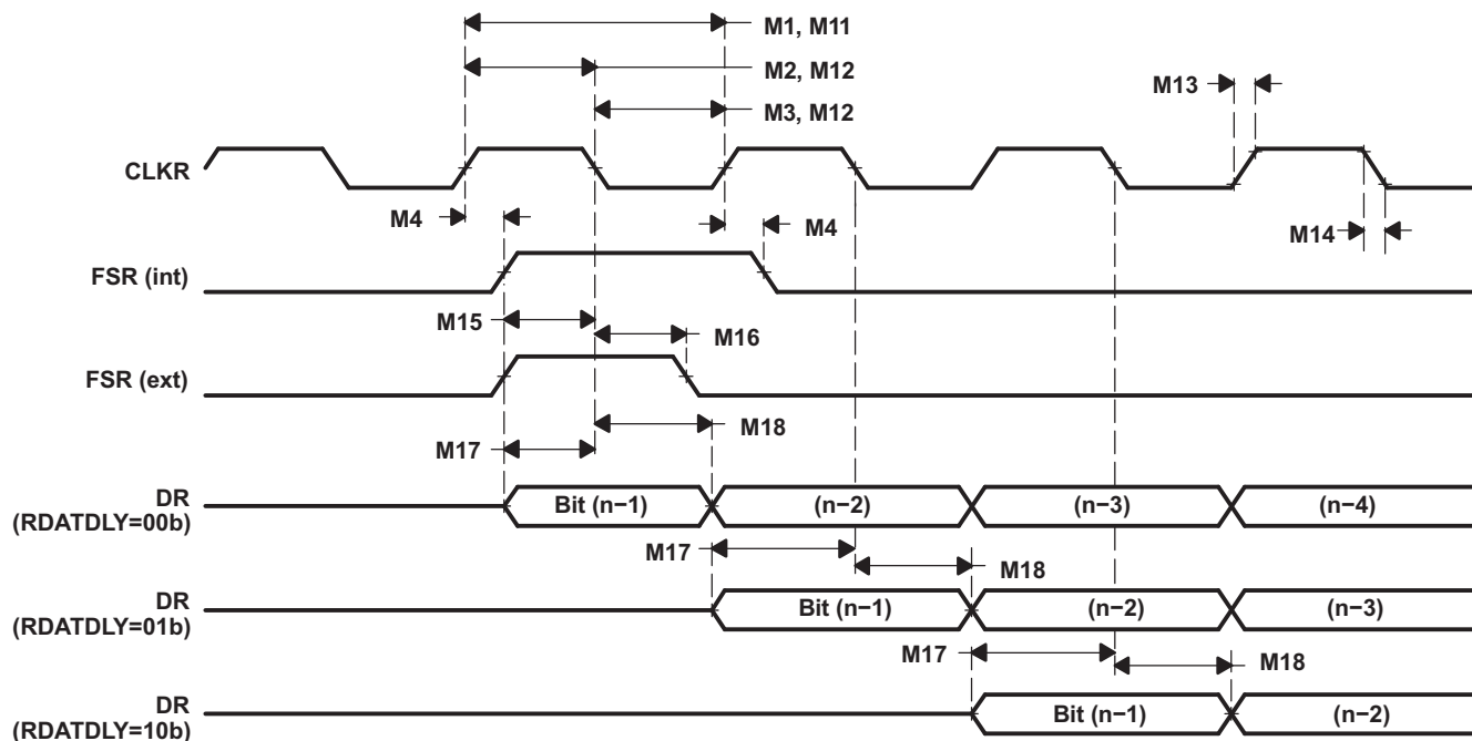
Figure 5-58. McBSP Receive Timing
