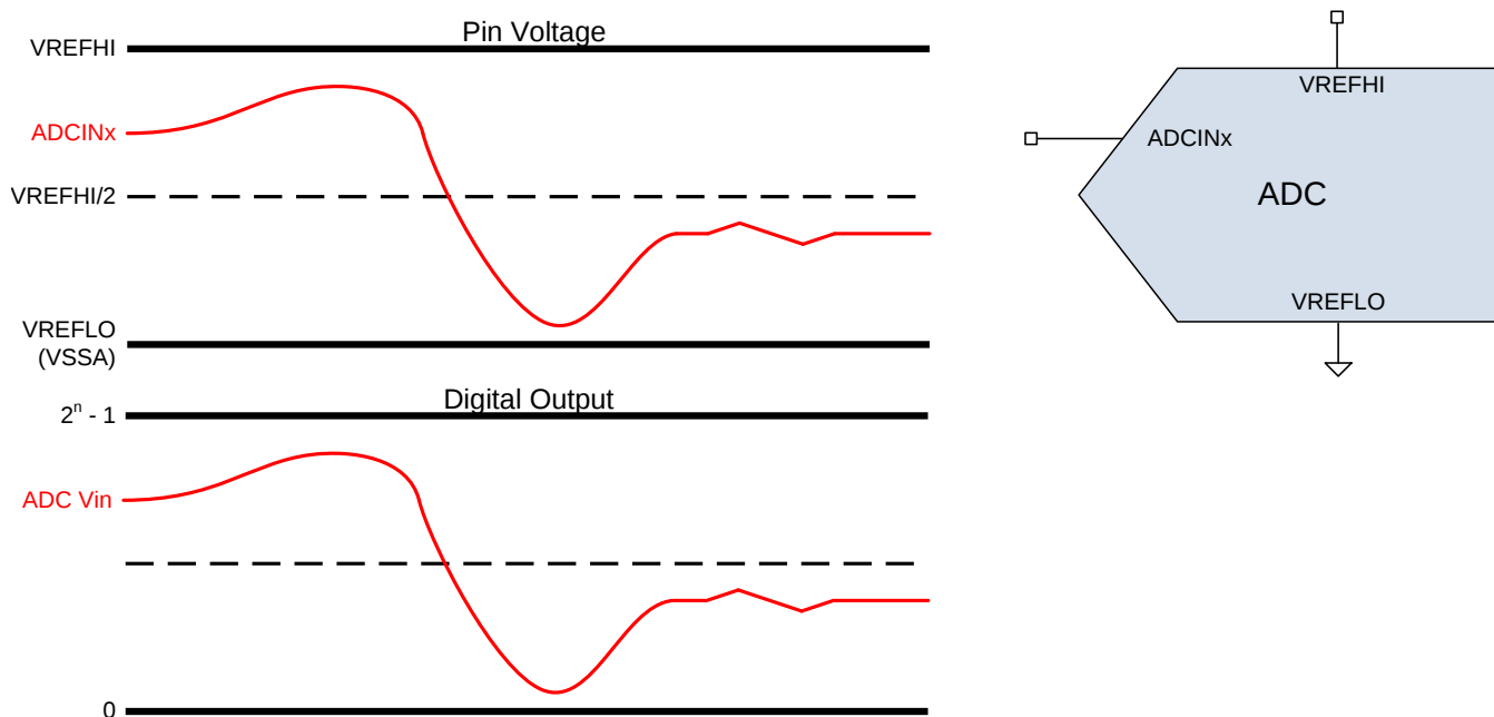
Figure 5-30. Single-ended Signaling Mode
