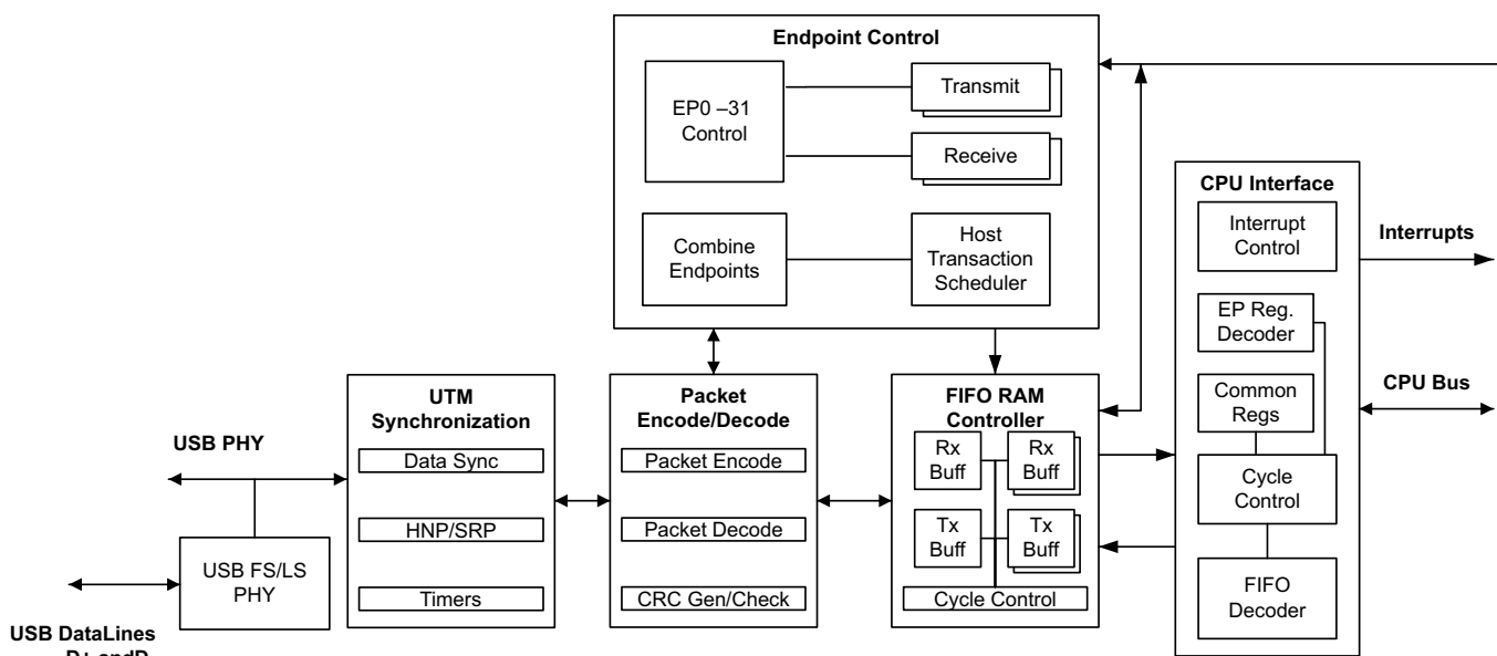
Figure 5-74. USB Block Diagram
