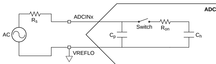
Figure 5-31. Single-Ended Input Model
