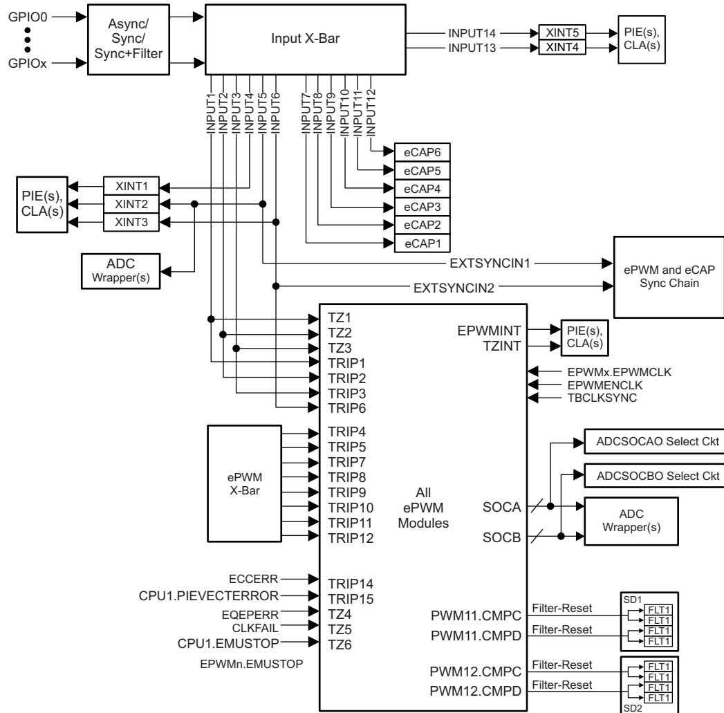
Figure 5-46. ePWM Trip Input Connectivity
