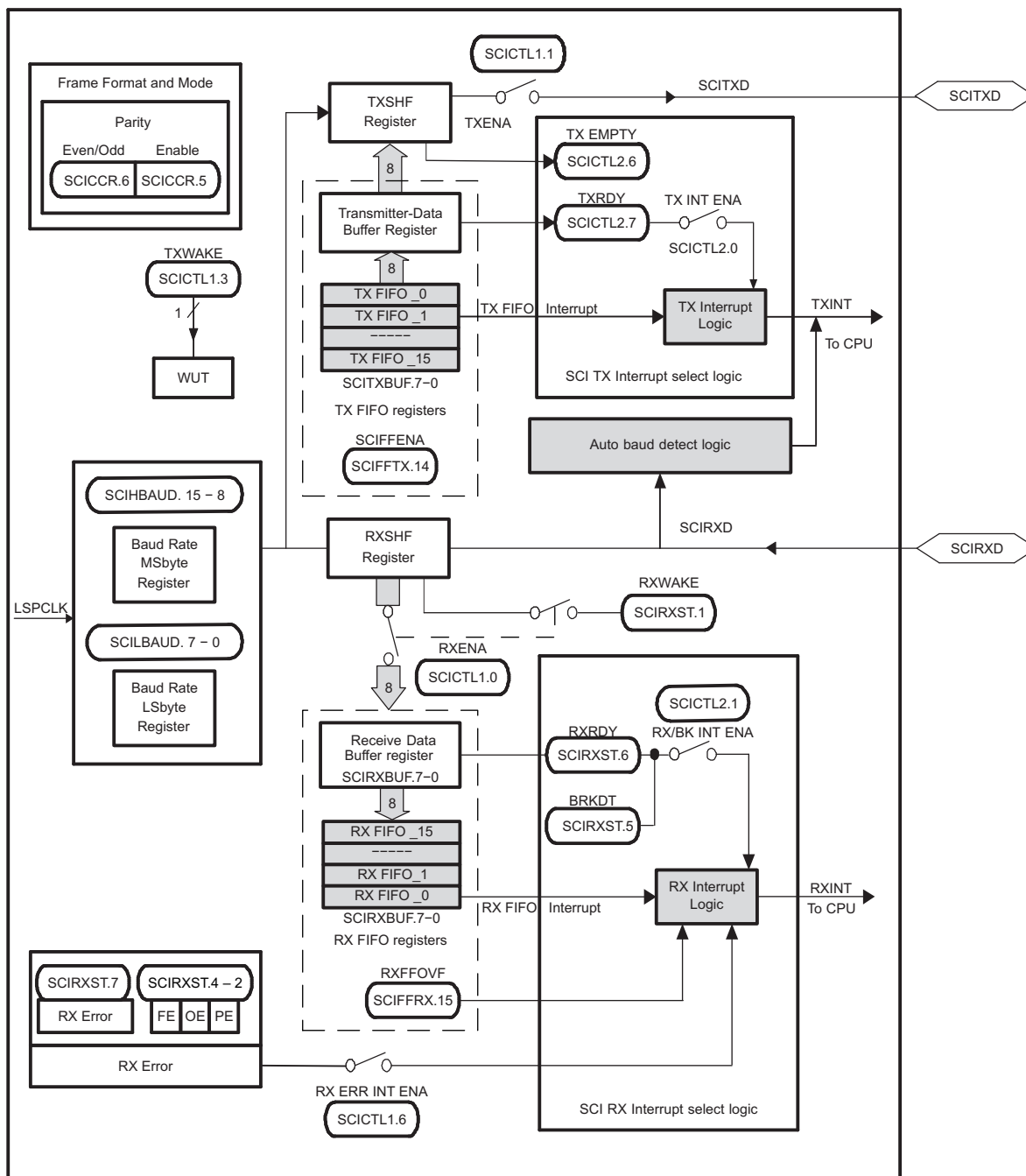
Figure 5-64. SCI Block Diagram
