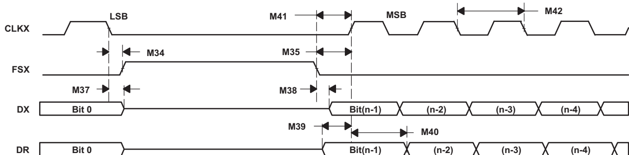
Figure 5-61. McBSP Timing as SPI Master or Slave: CLKSTP = 11b, CLKXP = 0
