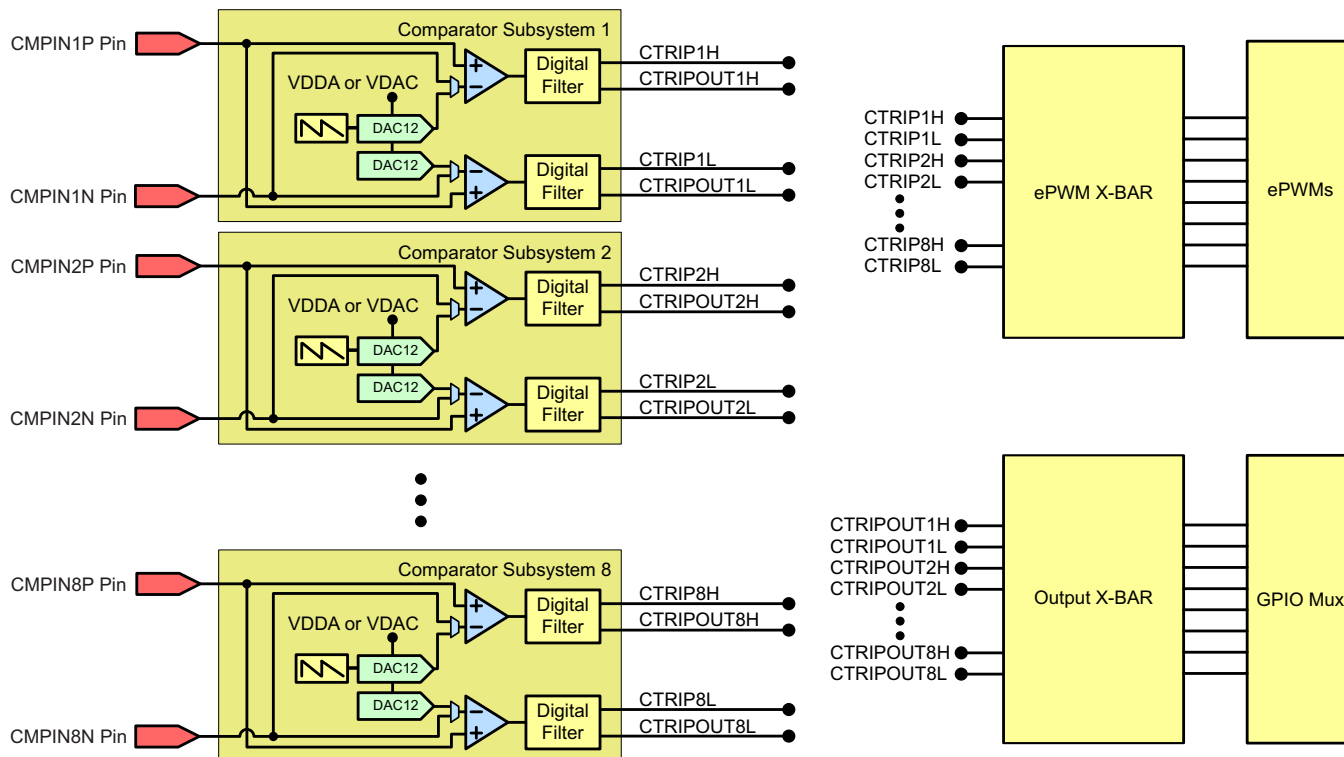
Figure 5-33. CMPSS Connectivity (176-Pin PTP)
