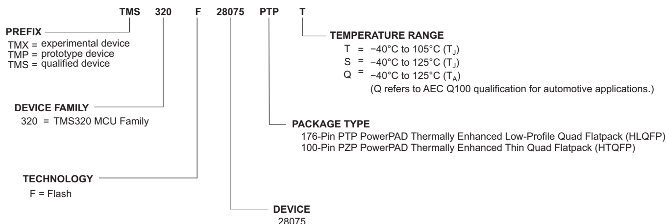
Figure 8-1. Device Nomenclature
