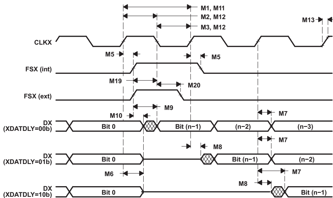
Figure 5-59. McBSP Transmit Timing
