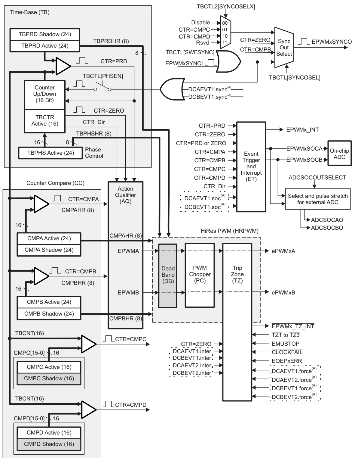
Figure 5-45. ePWM Submodules and Critical Internal Signal Interconnects
