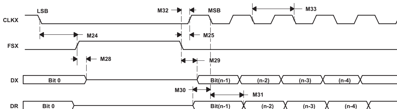
Figure 5-60. McBSP Timing as SPI Master or Slave: CLKSTP = 10b, CLKXP = 0
