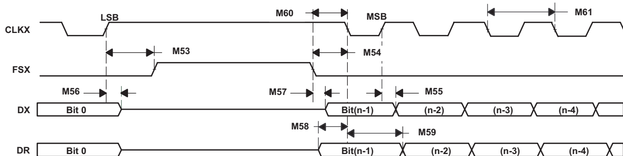
Figure 5-63. McBSP Timing as SPI Master or Slave: CLKSTP = 11b, CLKXP = 1
