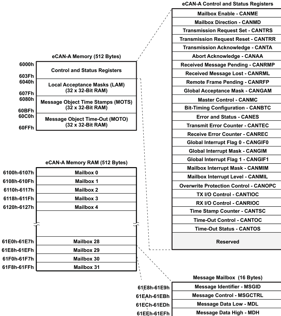
Figure 6-21. eCAN-A Memory Map
