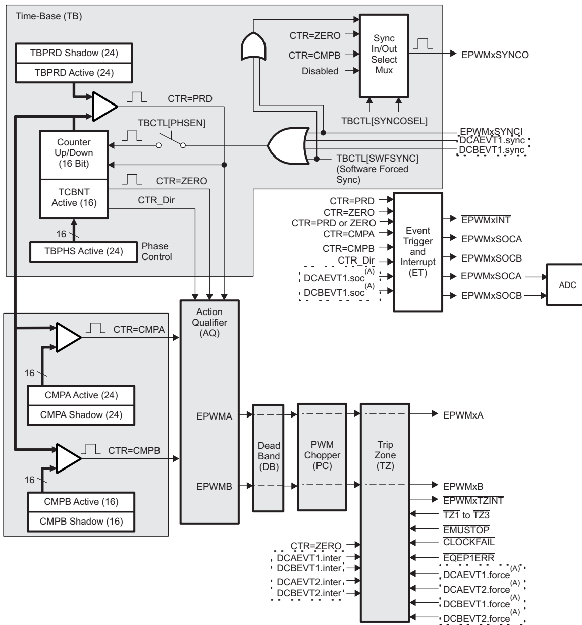
Figure 6-24. ePWM Sub-Modules Showing Critical Internal Signal Interconnections
