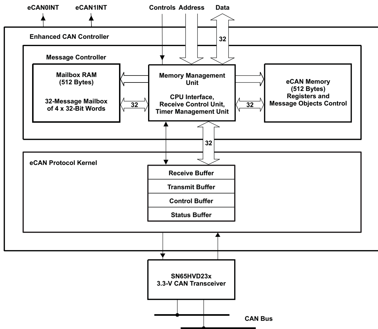
Figure 6-20. eCAN Block Diagram and Interface Circuit
