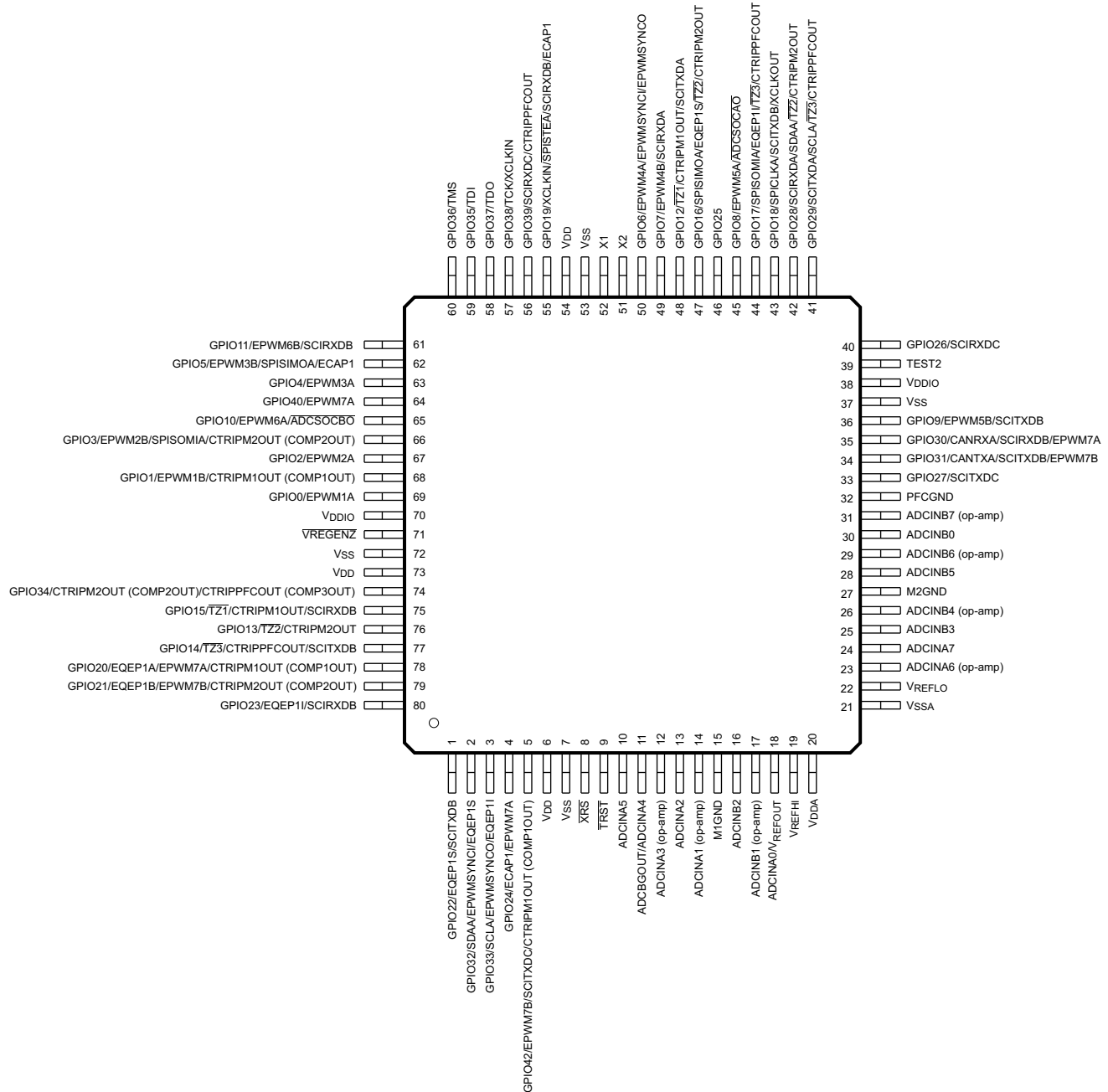
Figure 3-1. 2805x 80-Pin PN LQFP (Top View)
