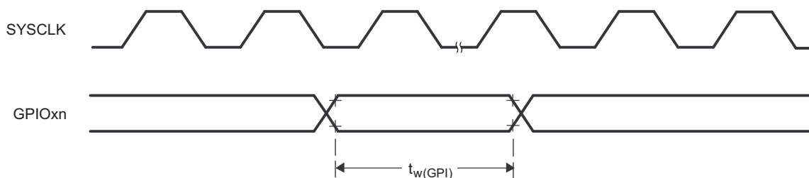
Figure 6-33. General-Purpose Input Timing
