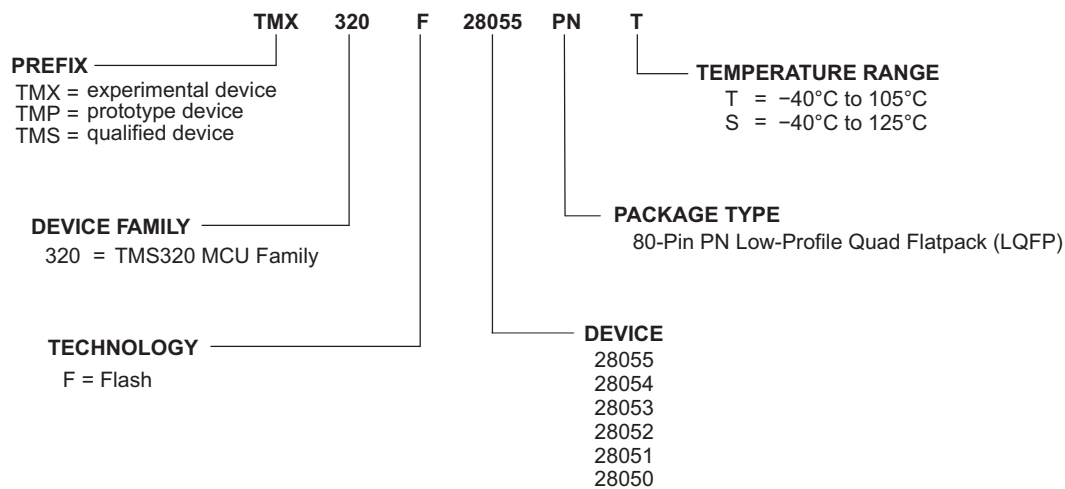
Figure 7-1. Device Nomenclature
