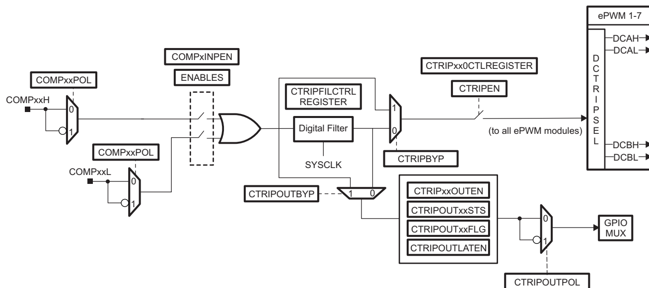
Figure 6-13. Comparator Trip/Digital Filter Subsystem
