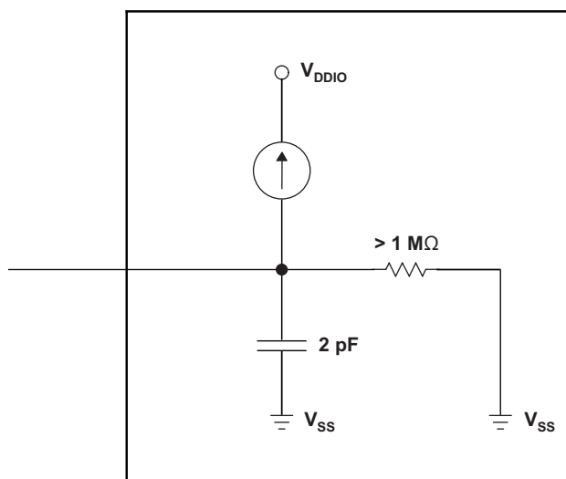
Figure 6-34. Input Resistance Model for a GPIO Pin With an Internal Pull-up
