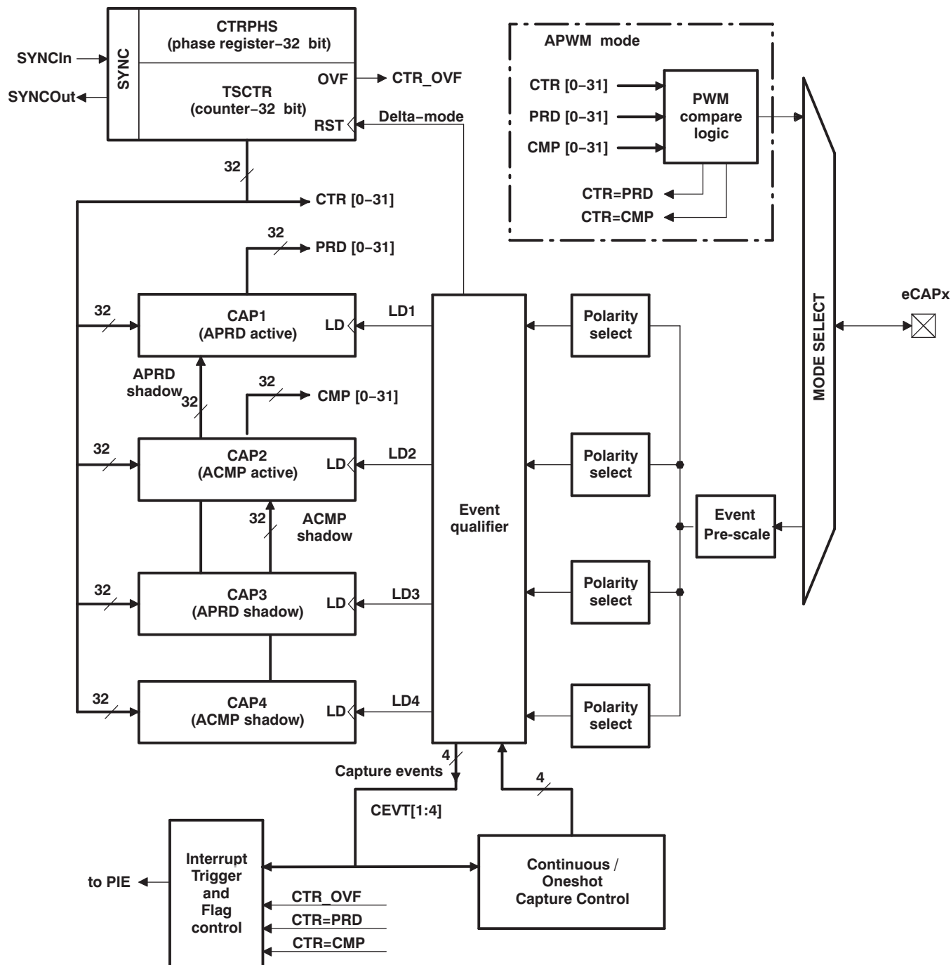
Figure 6-26. eCAP Functional Block Diagram
