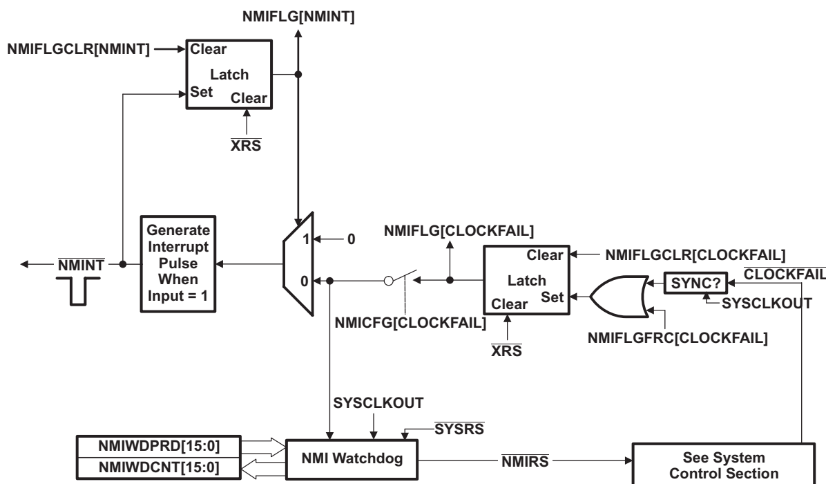
Figure 2-10. NMI-watchdog
