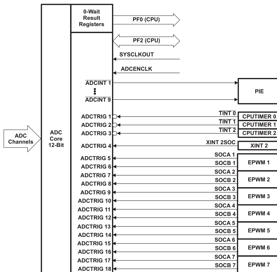
Figure 6-3. ADC Connections
