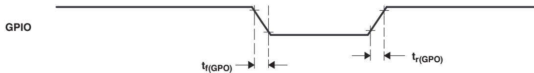
Figure 6-31. General-Purpose Output Timing
