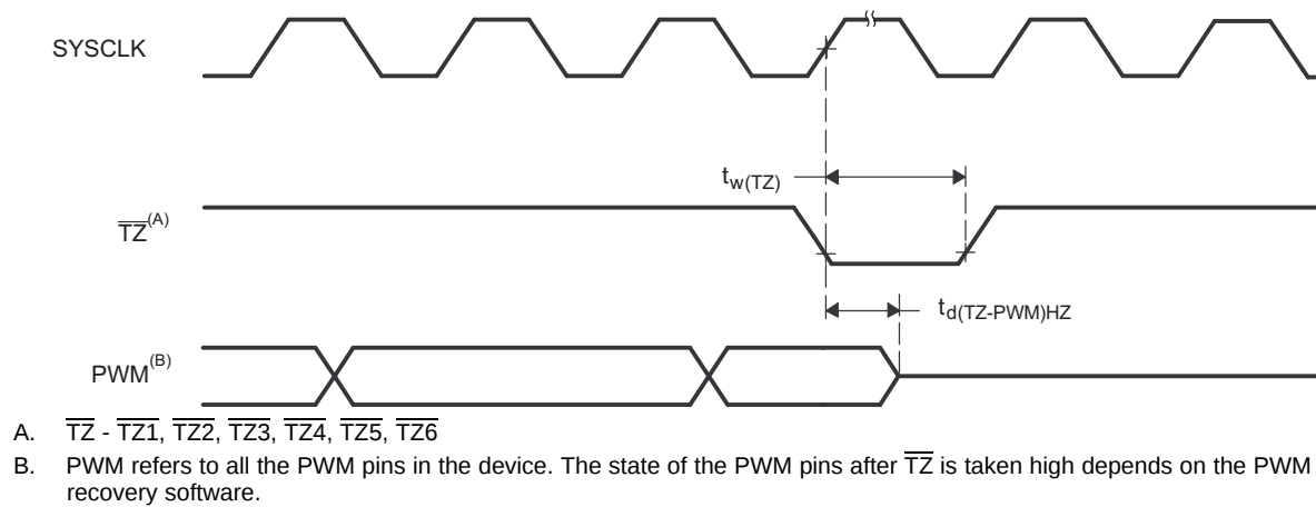
Figure 6-25. PWM Hi-Z Characteristics
