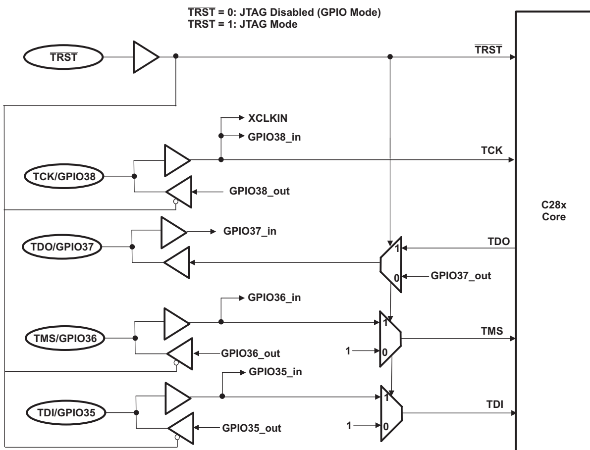
Figure 6-28. JTAG/GPIO Multiplexing
