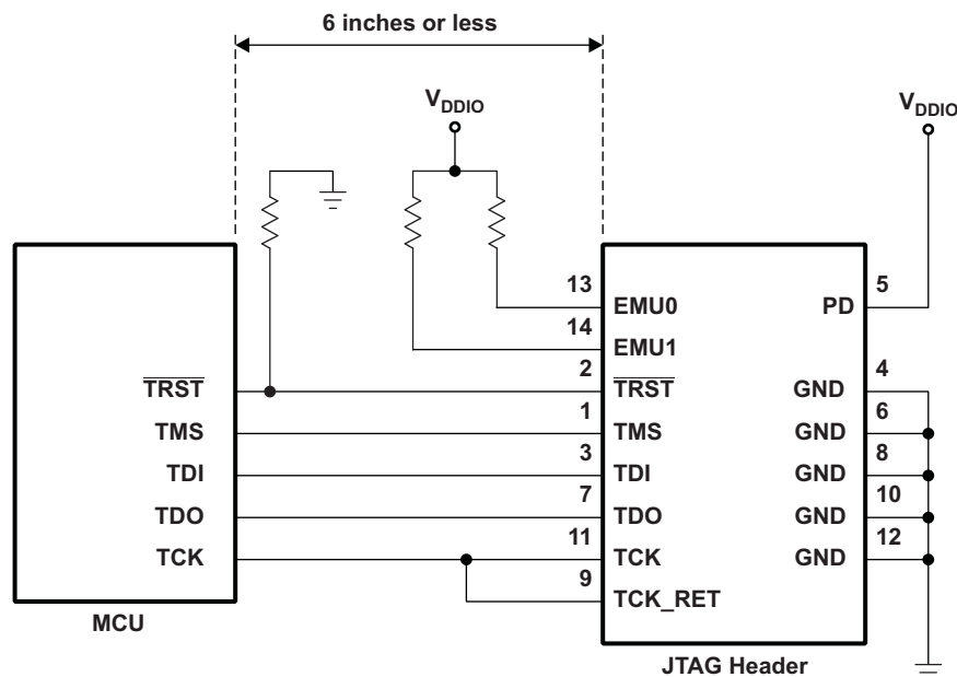
Figure 6-29. Emulator Connection Without Signal Buffering for the MCU
