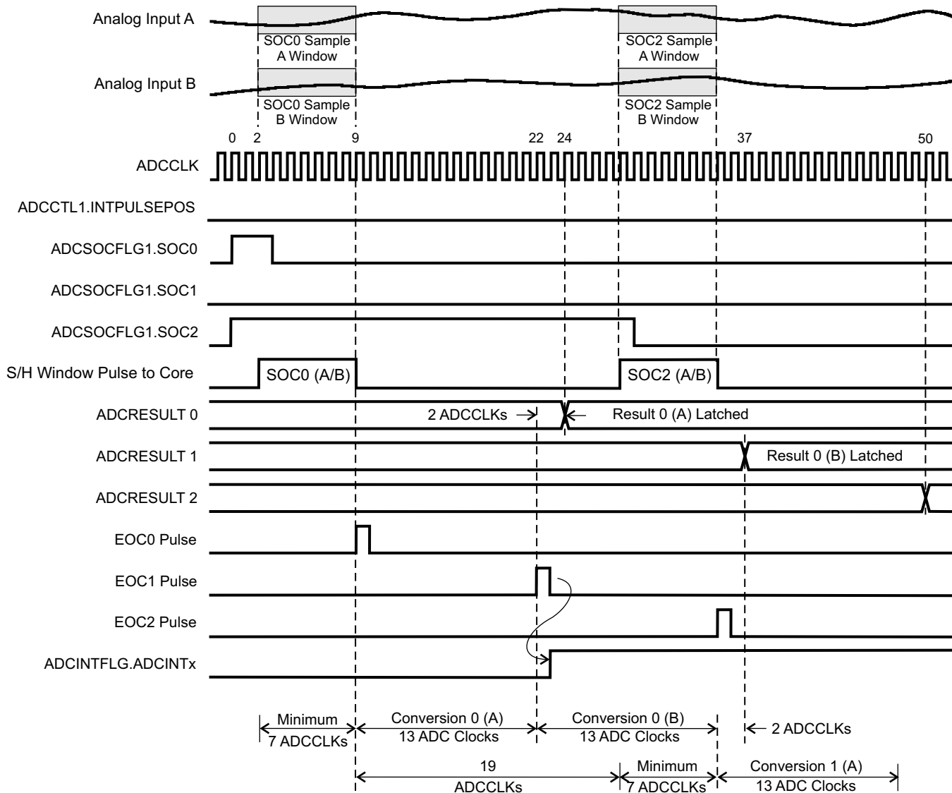
Figure 6-10. Timing Example for Simultaneous Mode / Early Interrupt Pulse
