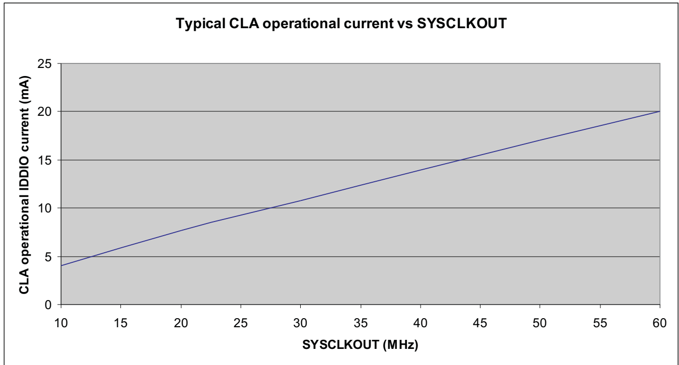
Figure 4-3. Typical CLA Operational Current Versus SYSCLKOUT
