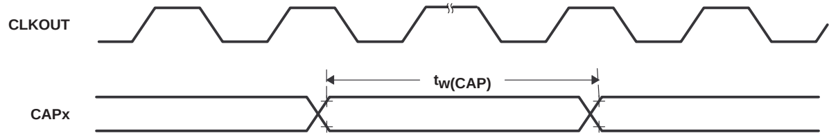
Figure 29. Capture Input and QEP Timing
