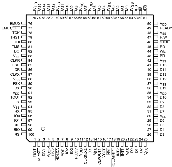
PZ PACKAGE
