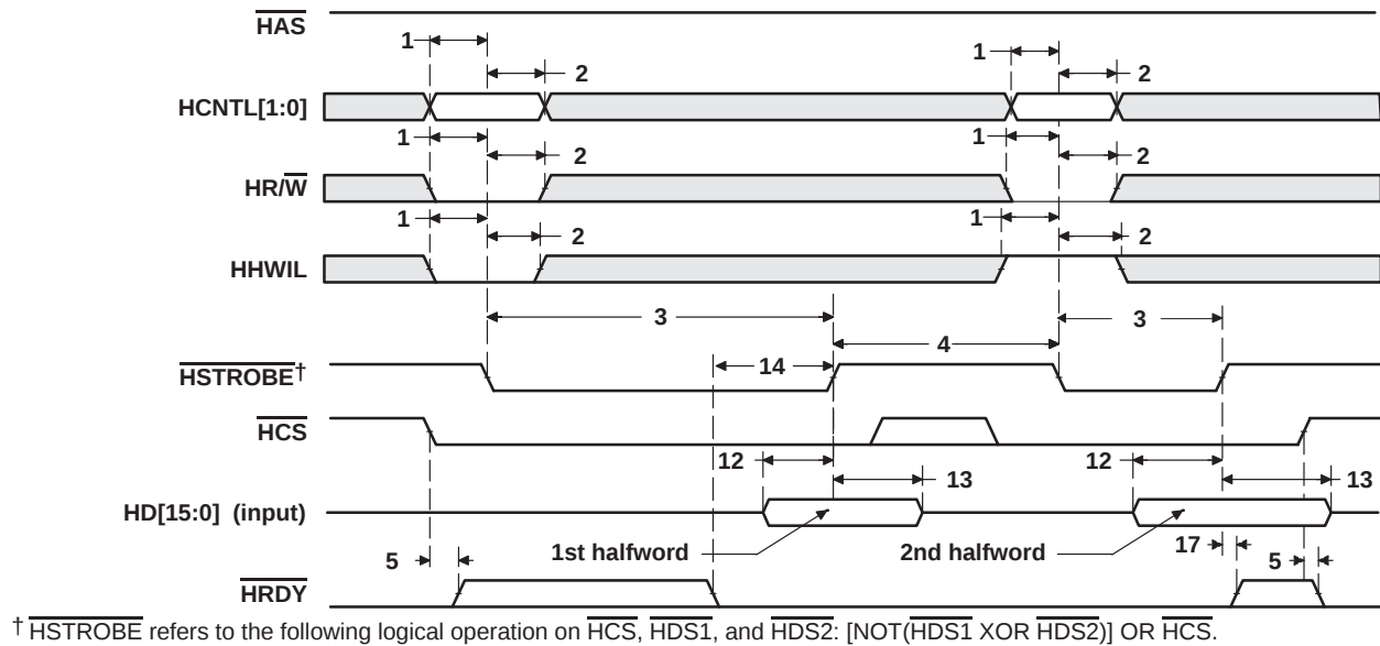
Figure 54. HPI Write Timing ( \overline{HAS} Not Used, Tied High)
