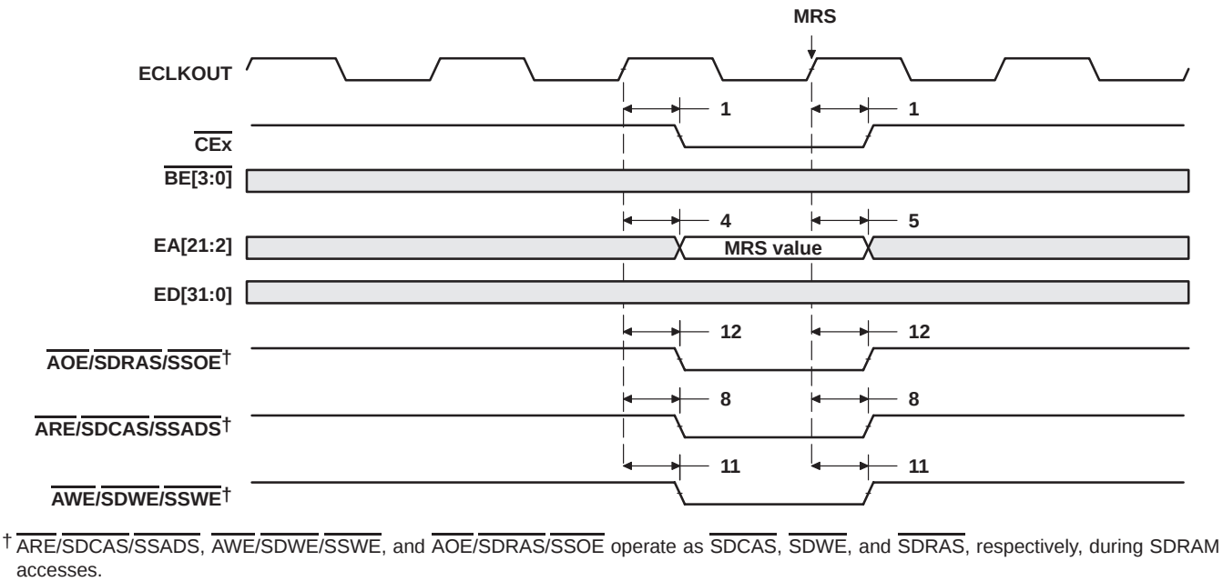
Figure 43. SDRAM MRS Command
