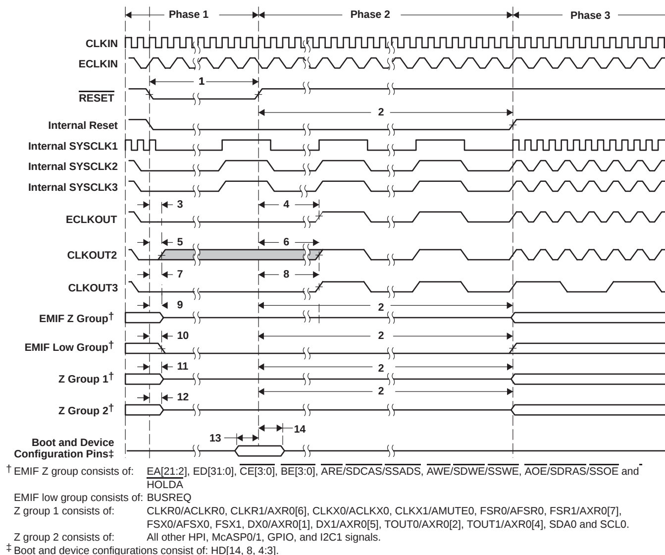
Figure 46. Reset Timing
