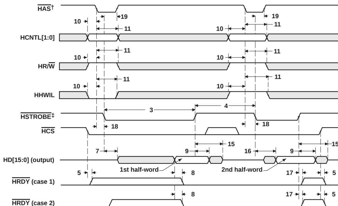
Figure 53. HPI Read Timing ( \overline{\text{HAS}} Used)
