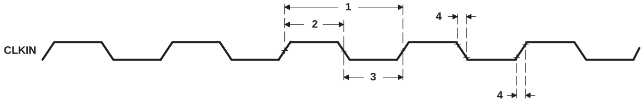
Figure 28. CLKIN Timings
