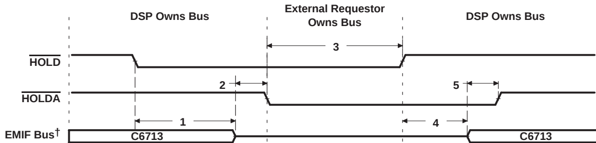
Figure 44. \overline{\text{HOLD}}/\overline{\text{HOLDA}} Timing
