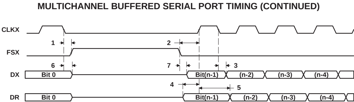
Figure 59. McBSP Timing as SPI Master or Slave: CLKSTP = 11b, CLKXP = 0
