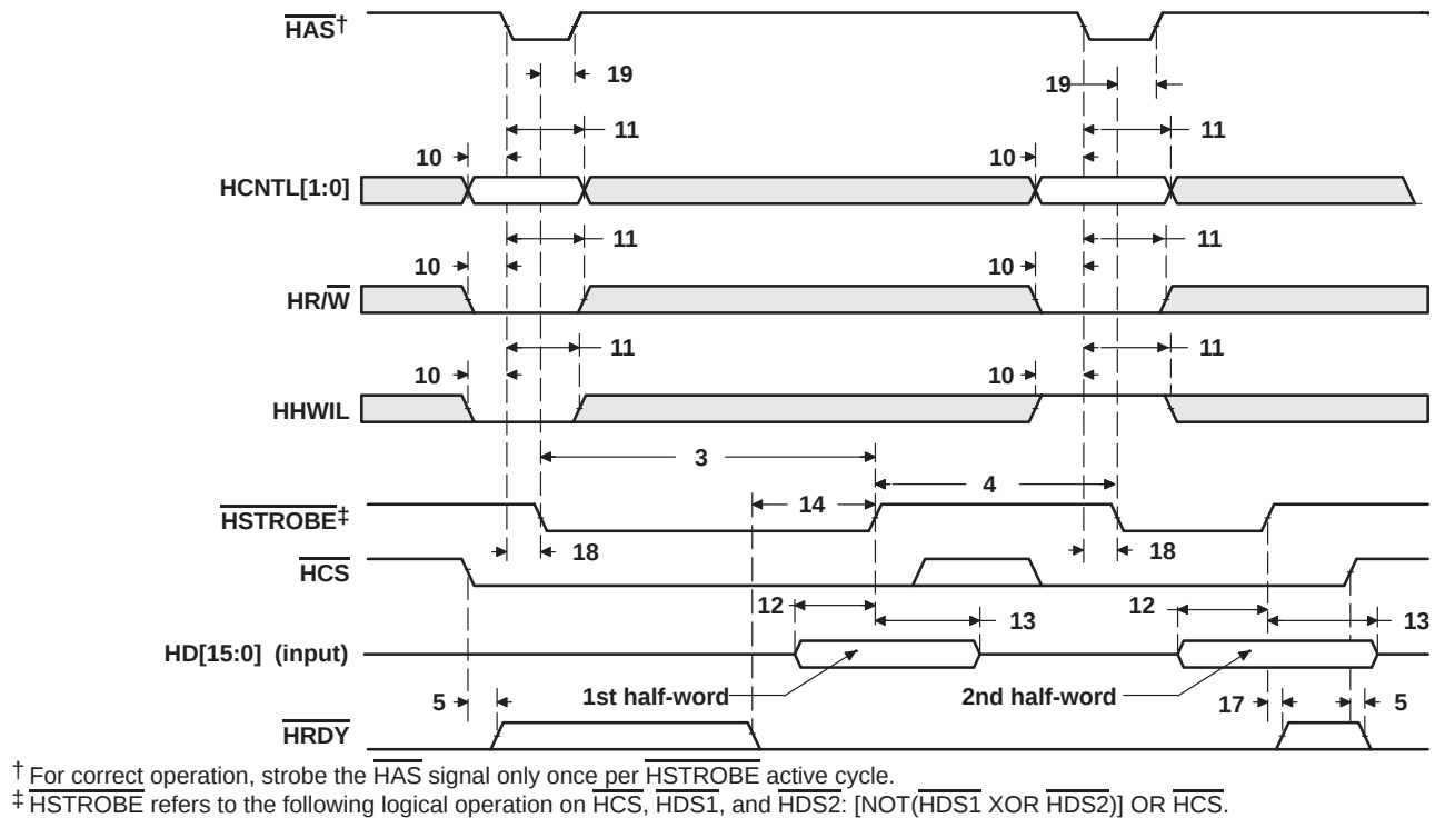
Figure 55. HPI Write Timing ( \overline{HAS} Used)
