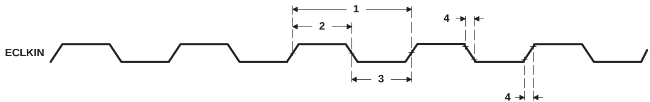
Figure 31. ECLKIN Timings
