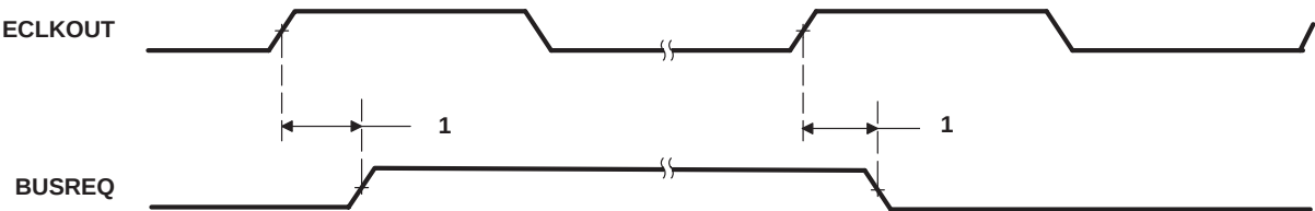
Figure 45. BUSREQ Timing
